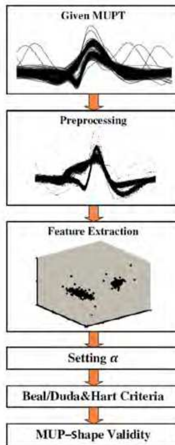
Fig. 6. An overview of the MUP-shape validation system.
