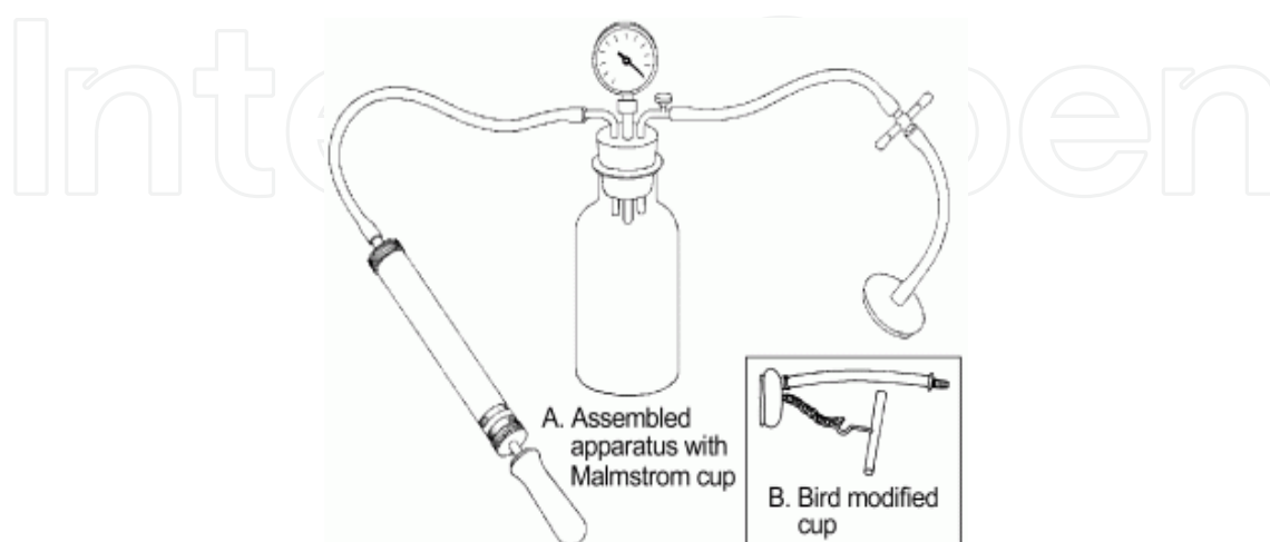
Fig. 2. A Malmstrom's vacuum extractor with its essential components. Inset: Bird's modification of metal cup
