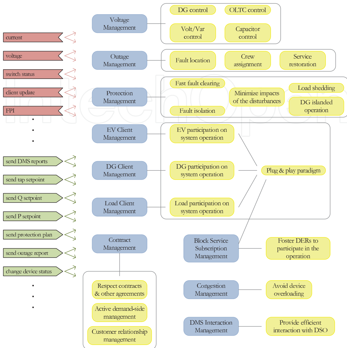
Fig. 6. Role overview for the agent-based architecture.
