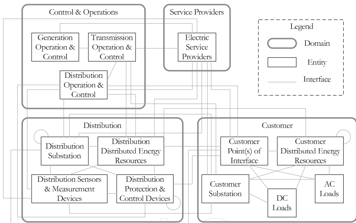
Fig. 1. Distribution grid interoperability perspective. Adapted from (IEEE P2030, 2011).
