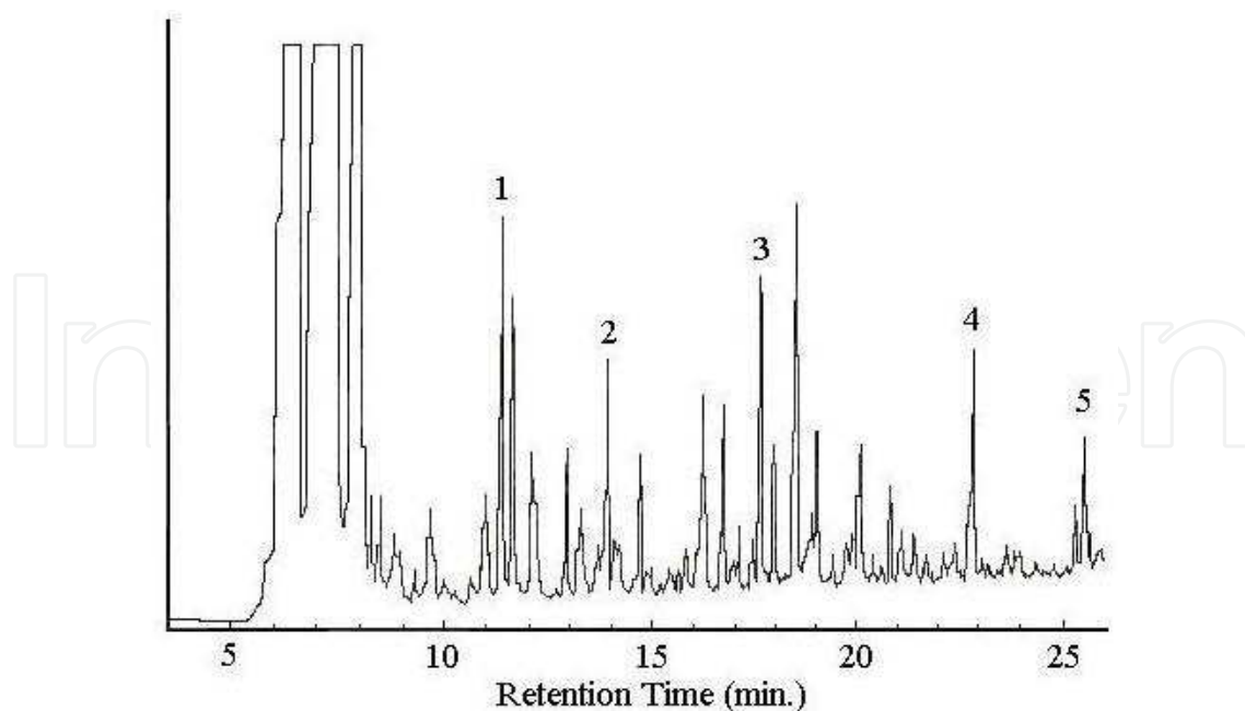
Fig. 3. Gas Chromatograms of all components from root exudate of strawberry plants adsorbed and released from AC. Methyl esters of lactic acid (peak 1), benzoic acid (peak 2), succinic acid (peak 3), adipic acid (peak 4) and p-hydroxy benzoic acid (peak 5) are identified based on known standard retention times.
