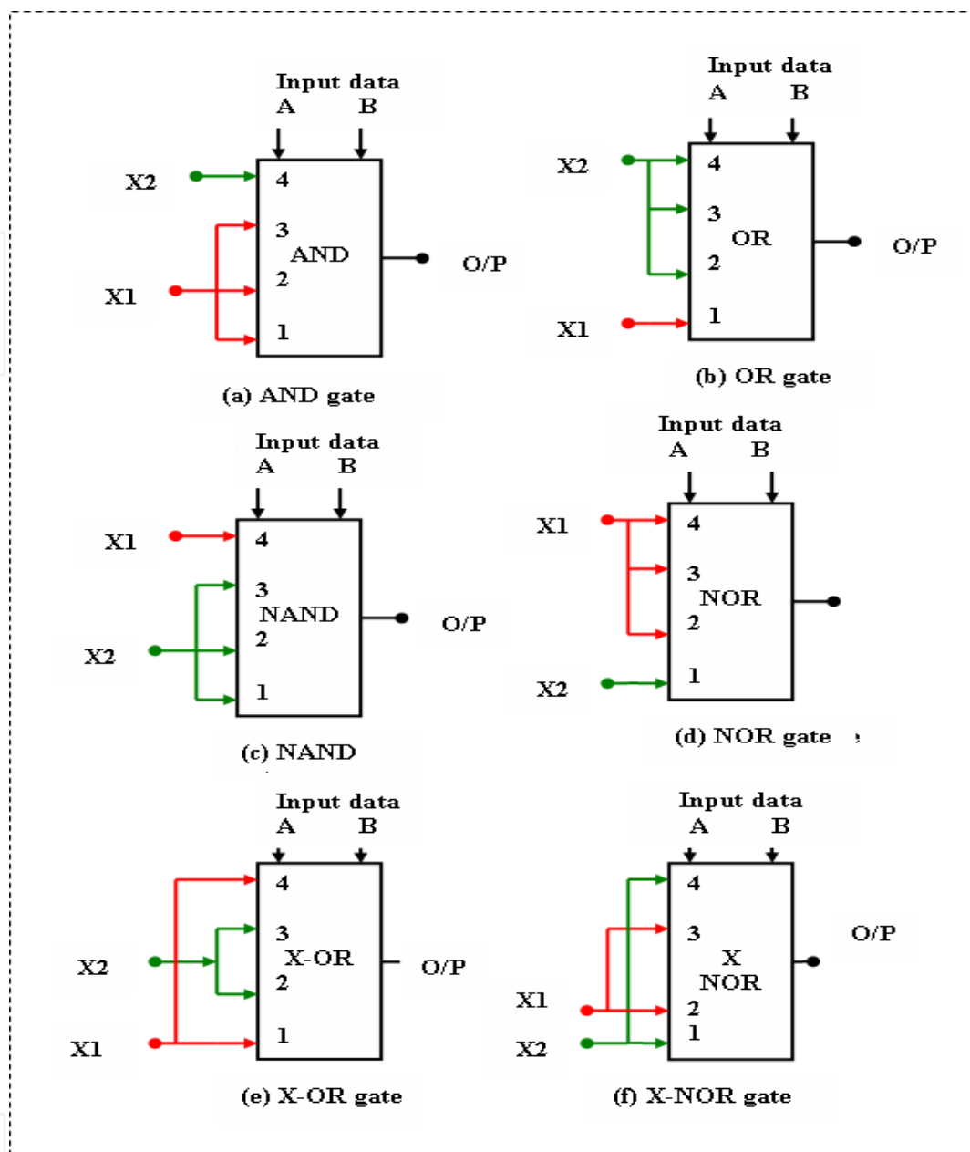
Fig. 4. Block diagram of different logic units
