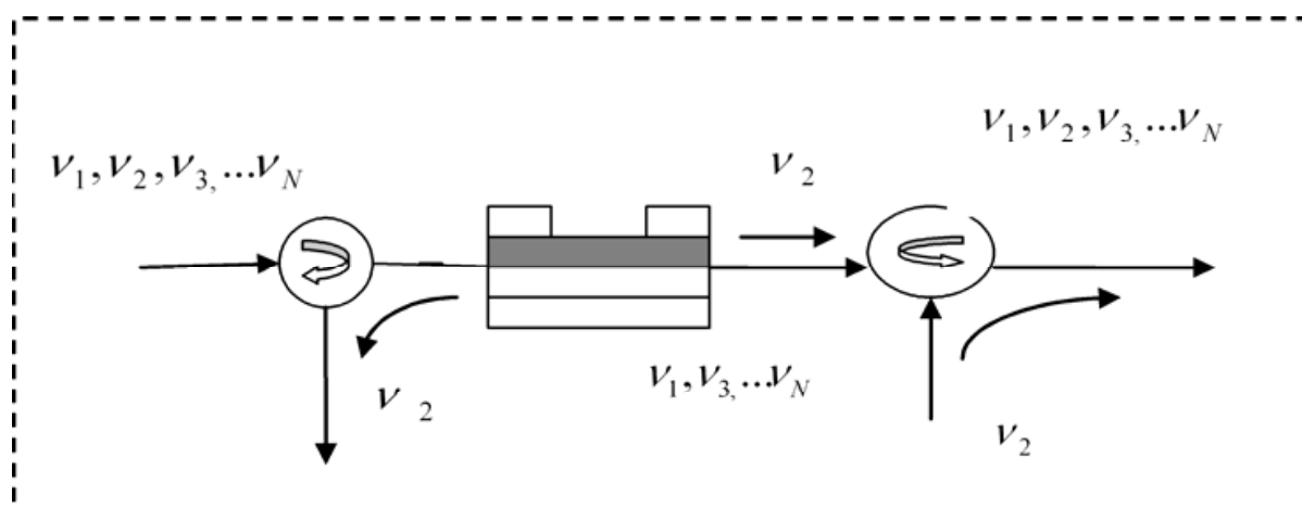
Fig. 1(b). SOA based add/drop multiplexer
