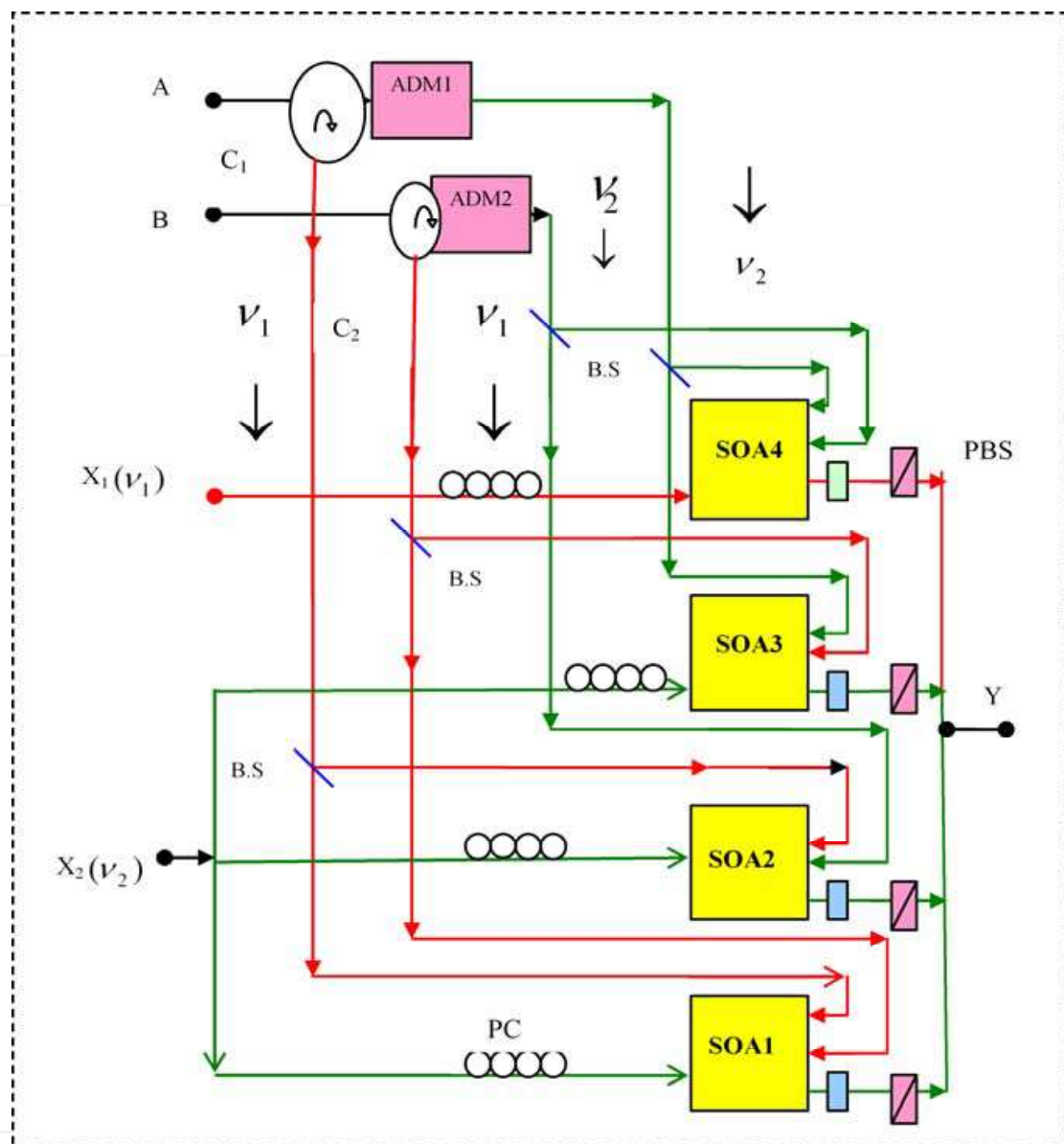
Fig. 3. Scheme of implementing frequency encoded NAND logic operation
