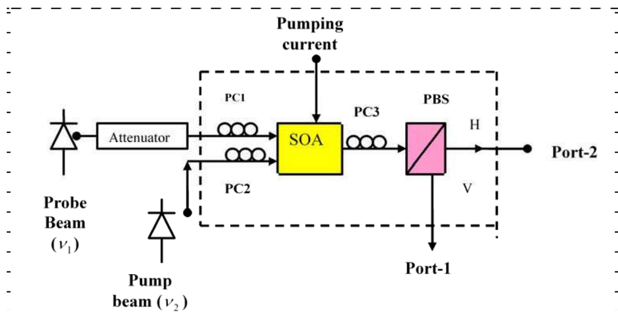
Fig. 1(c). SOA acting as a polarization switch
