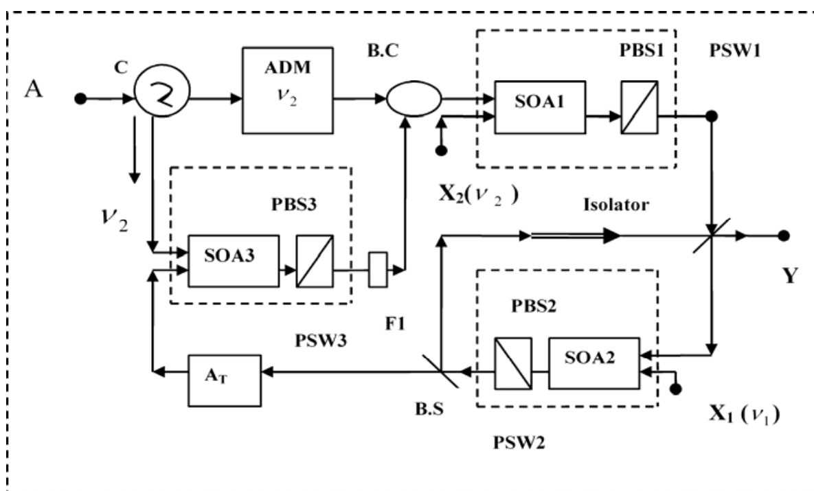
Fig. 5. Frequency encoded single bit memory circuit
