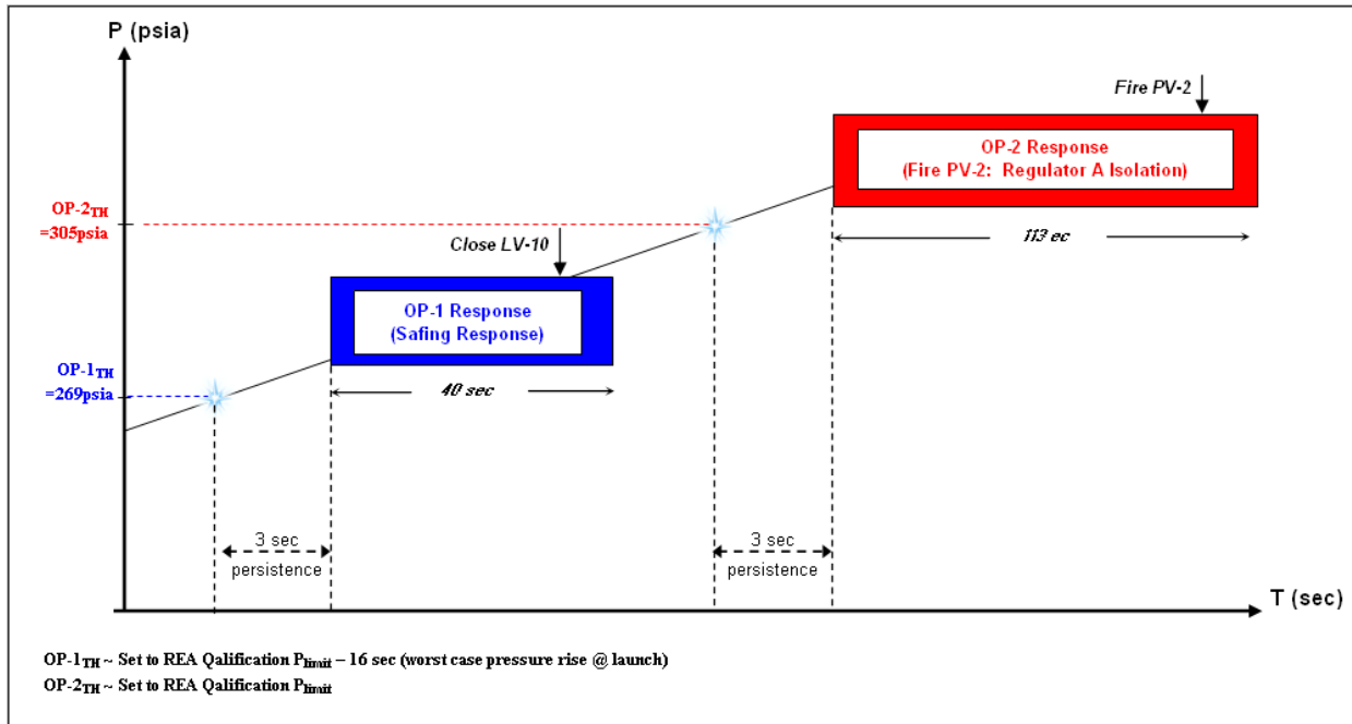
Fig. 12. OP-1 & OP-2 Monitor and Response Configuration.
