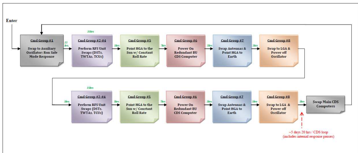
Fig. 7. Cassini's Command Loss Response Chain for One CDS Cycle (Endless Loop Response).
