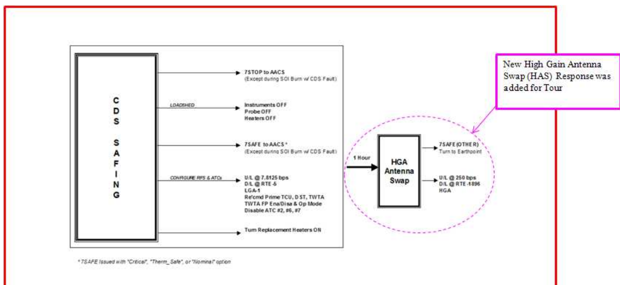
Fig. 9. New HGA Response was added in 2003; Configured to Run 1 hr. after Safing Response Executes.
