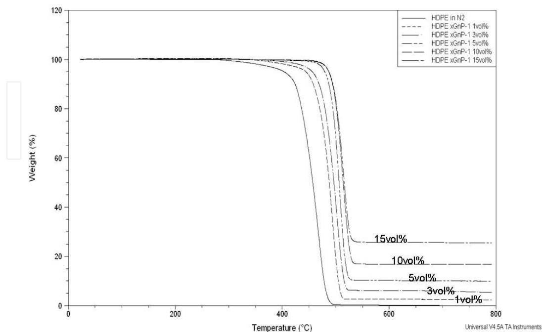
Fig. 8. TGA curves of HDPE and HDPE/GNP-1 nanocomposites.
