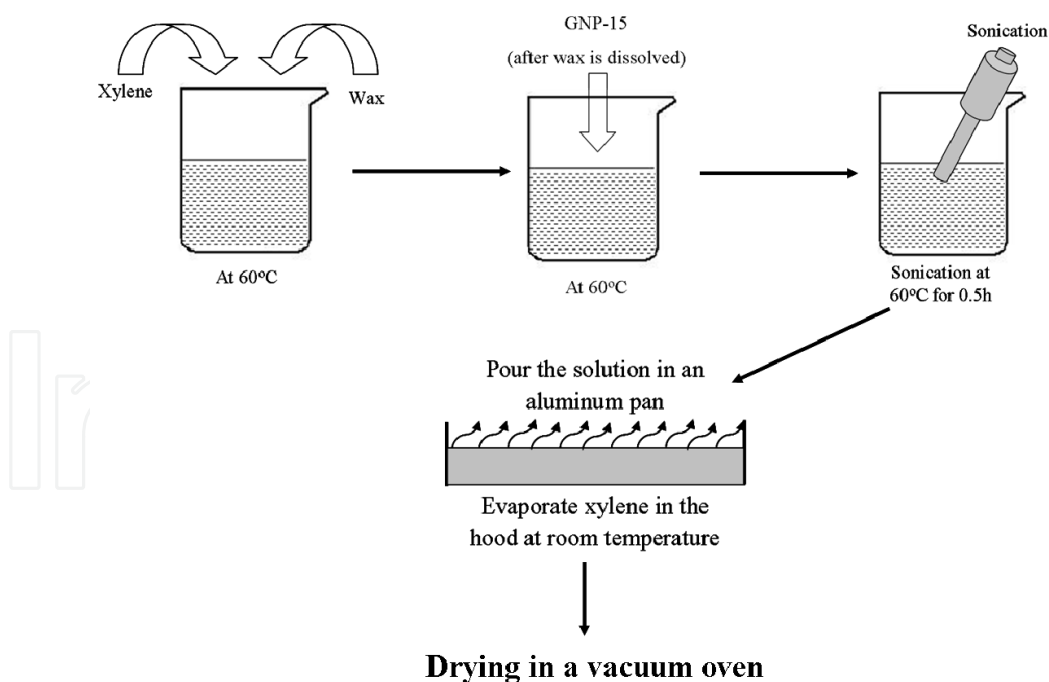
Fig. 2. The procedure of producing wax coated GNP-15.
