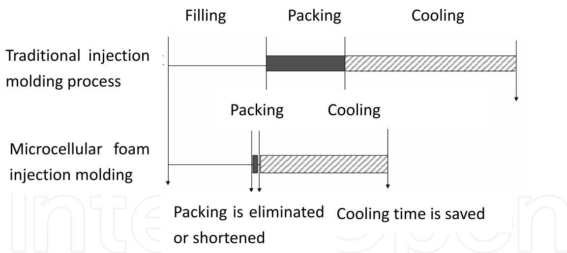
Fig. 1-4. Comparison between microcellular foam injection molding process cycle and traditional injection process.
