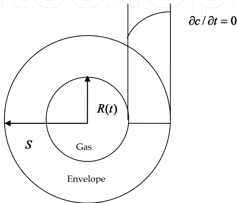
Fig. 2-5. Schematic of the unit cell model.
