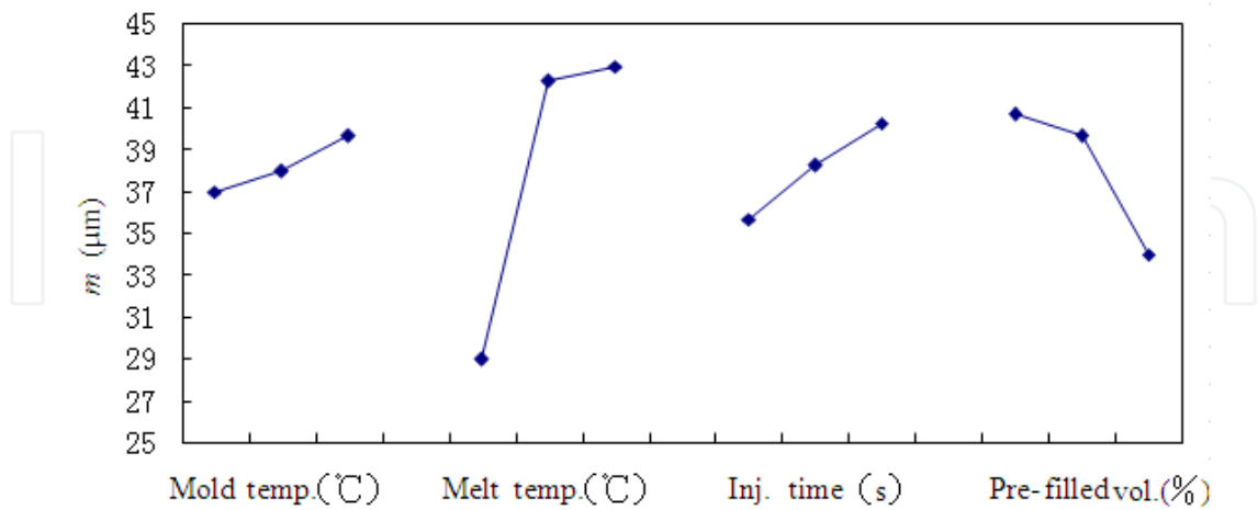
Fig. 2-7. Effect of each process parameter on cell size.
