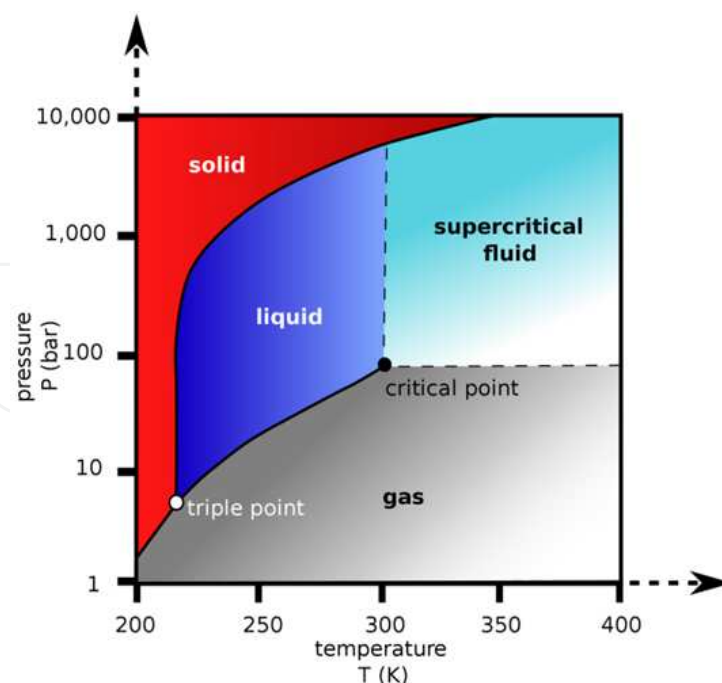
Fig. 2-1. Carbon dioxide pressure-temperature phase diagram [30].
