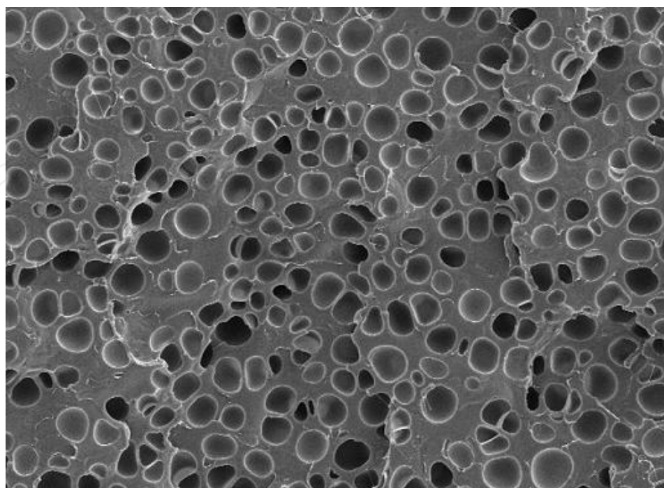
Fig. 1-1. Electron micrographs of microcellular polystyrene scanning sample [2].
