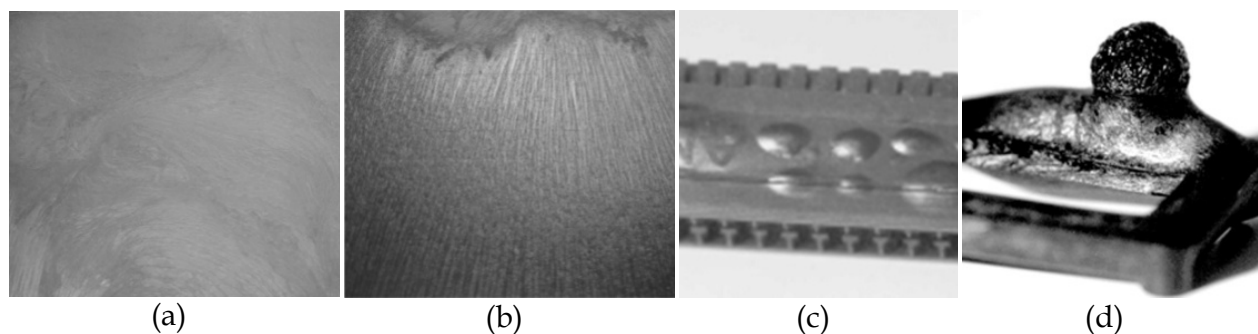
Fig. 1-6. Surface defects of microcellular foam injection molding parts (a) swirl mark [14] ; (b) silver streak [14] ; (c) surface blistering [15] ; (d) post-blow [15] .
