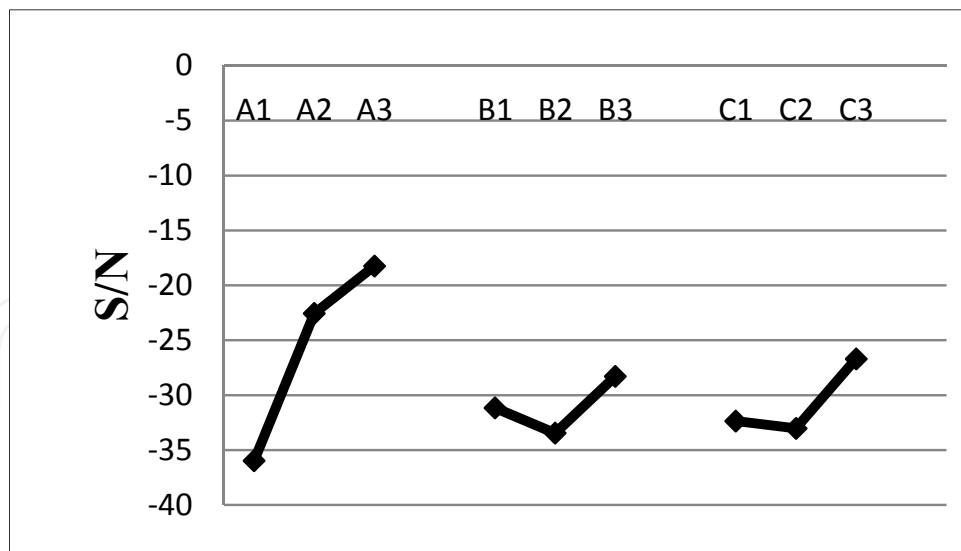
Fig. 2-3. Effect of each factors on S/N ratio.
