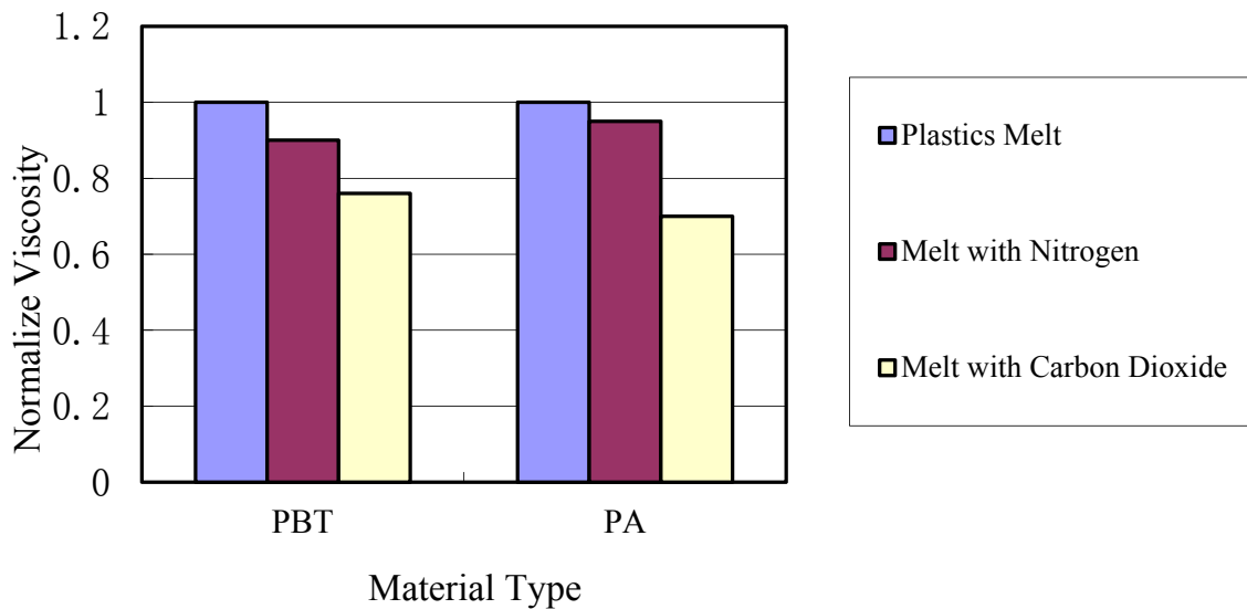
Fig. 1-3. Effect of SCF on melt viscosity [4].
