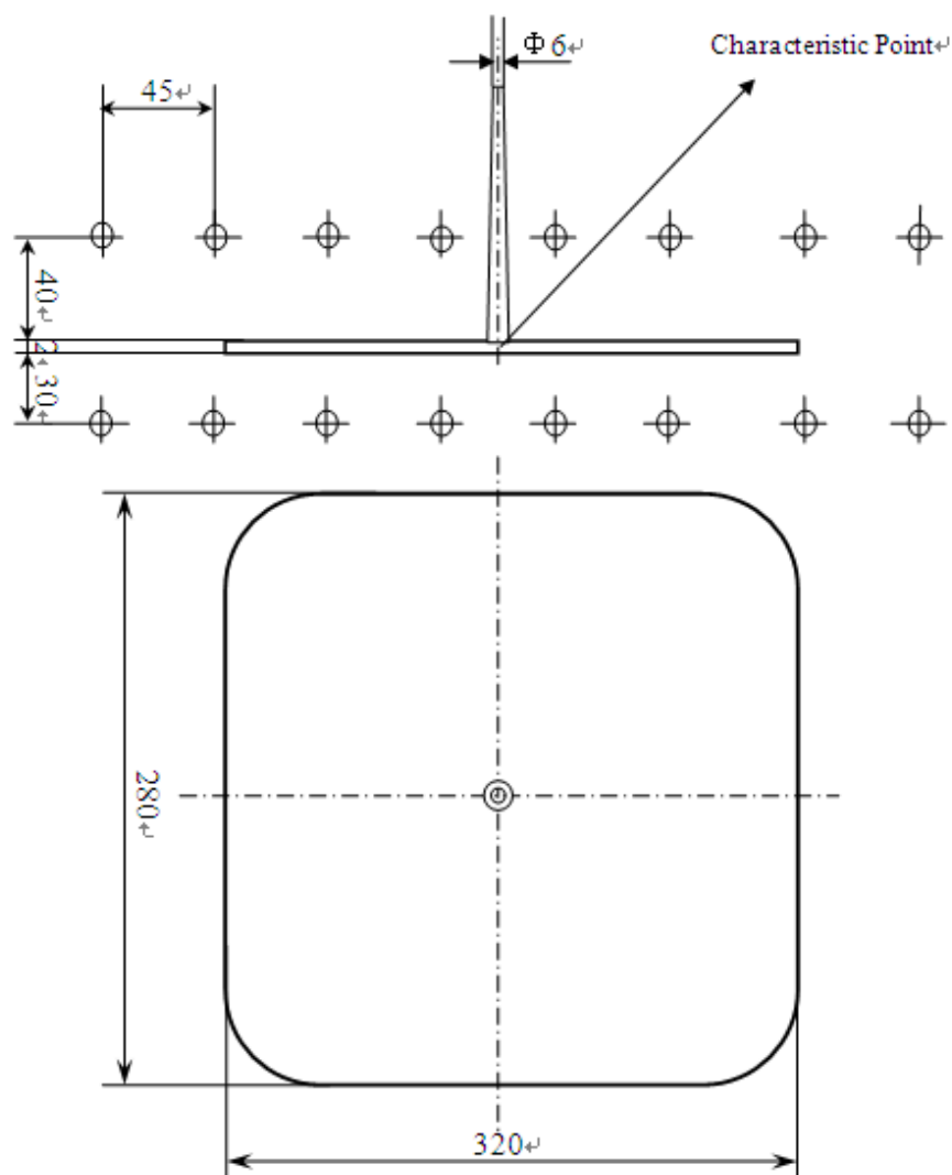
Fig. 2-6. Experiment model.
