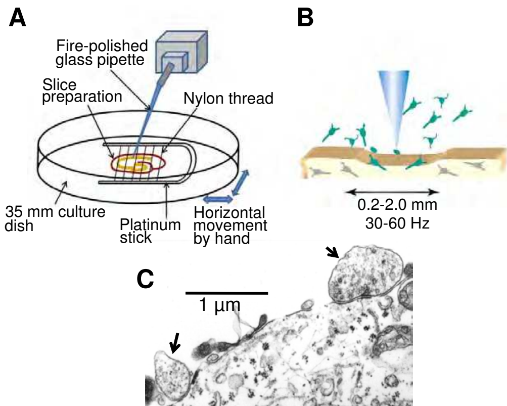
Fig. 1. Mechanical isolation of single CNS neurons
