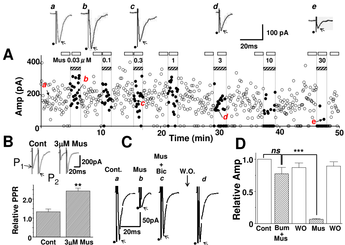
Fig. 6. Glutamatergic evoked EPSCs
