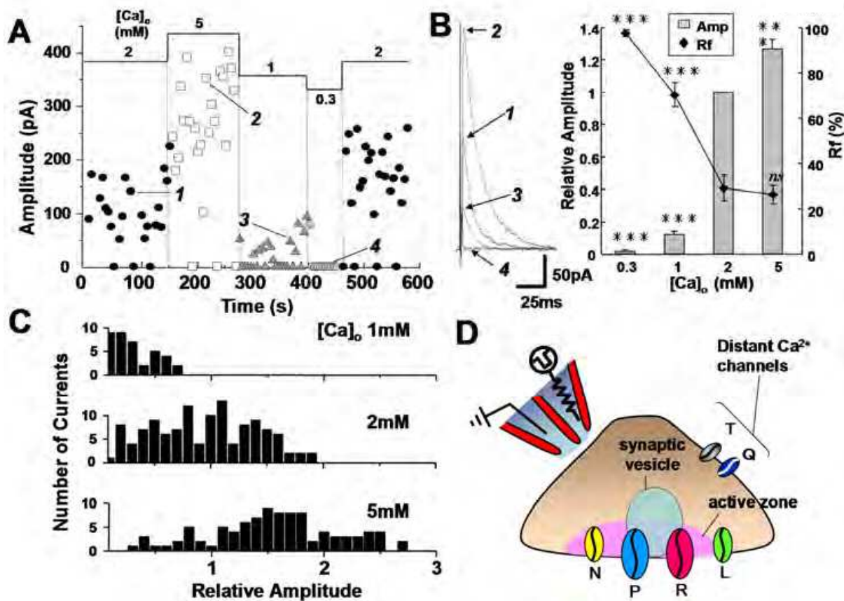
Fig. 5. Effects of changes in the external \text{Ca}^{2+} concentration ( [\text{Ca}^{2+}]_o ) on glycinergic eIPSCs from the spinal SDCN neuron
