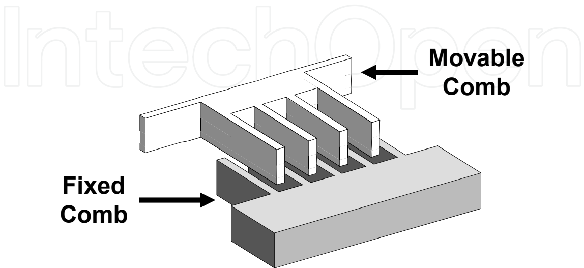
Fig. 2.2. Schematic of a vertical combdrive actuator
