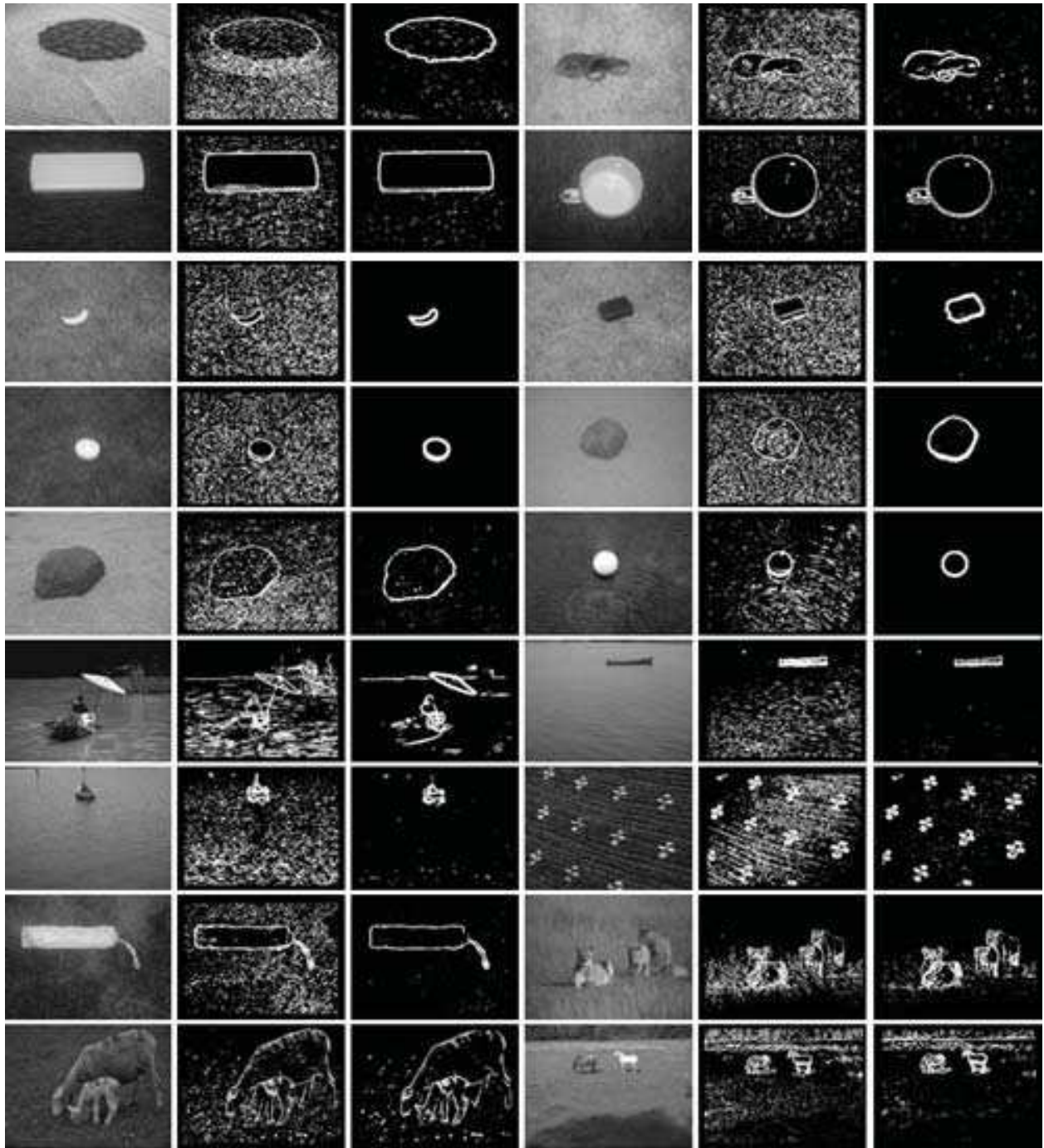
Fig. 12. Segmentation comparison . Column 1 and 4 : Images with obvious boundaries.(some from Berkeley Dataset Martin et al. (2001)). Column 2 and 5 : Thresholded by OT. Column 3 and 6 : Thresholded at Scale and OT corresponding to inflection of OT.
