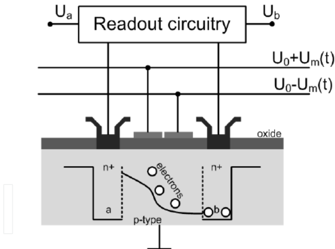
Fig. 1. Cross section of a typical PMD pixel
