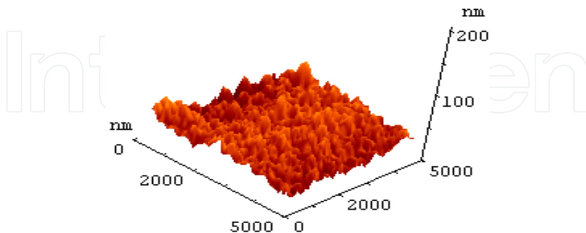
Fig. 8. AFM image of ZnO on PPC substrate (rms =10 nm)
