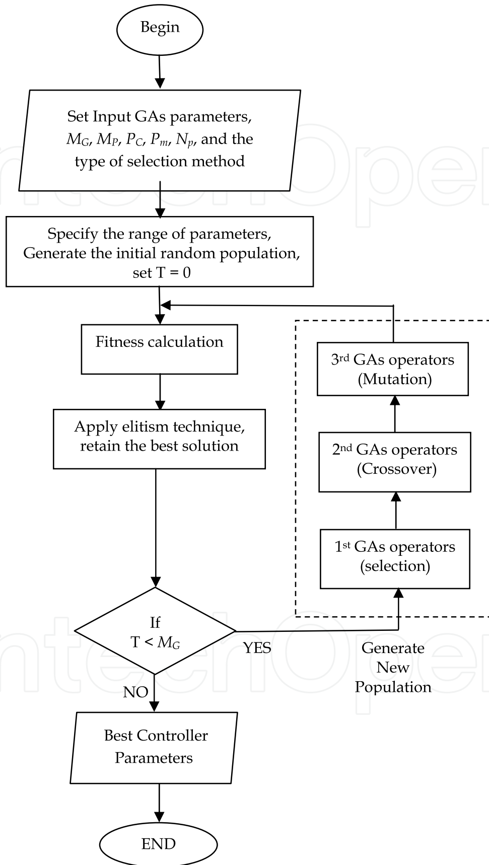
Fig. 3. Flowchart of Genetic PID Controller Algorithm
