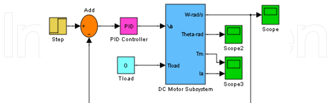
Fig. 12. Speed Control of DC Motor System with PID Controller.
