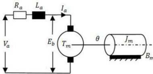
Fig. 9. Separately excited DC motor.
