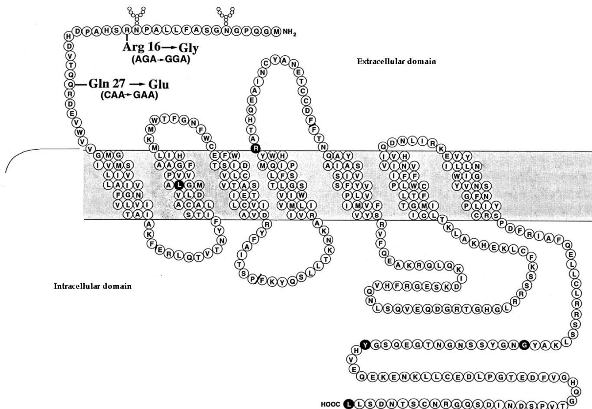
Fig. 1. Most common clinically relevant polymorphisms of the \beta 2-adrenoreceptor (Liggett, 1997-changed). Black - nucleic acid deviations from wild type not resulting in nucleotide changes.
