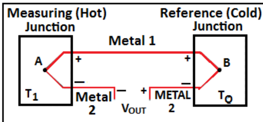
Fig. 3. Voltage measurement arrangement between two junctions
