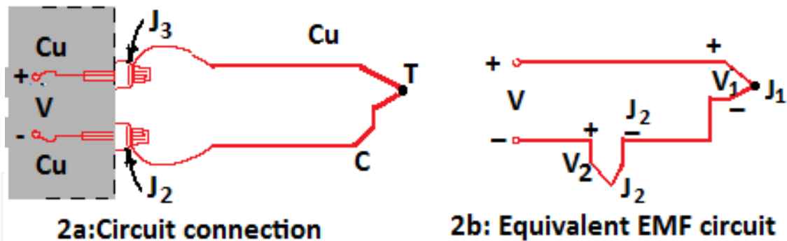
Fig. 2. Measuring Seebeck voltage
