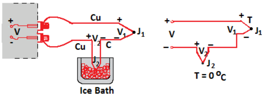
Fig. 4. External reference junction
