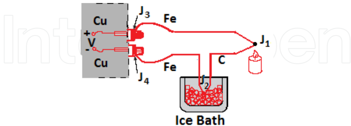
Fig. 5. An Iron- constantan couple
