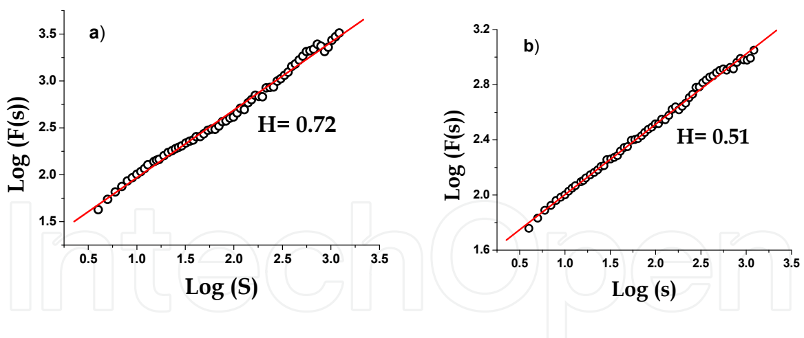
Fig. 6. a) Hurst exponent for Curitiba station. b) The exponent H for the shuffled series.
