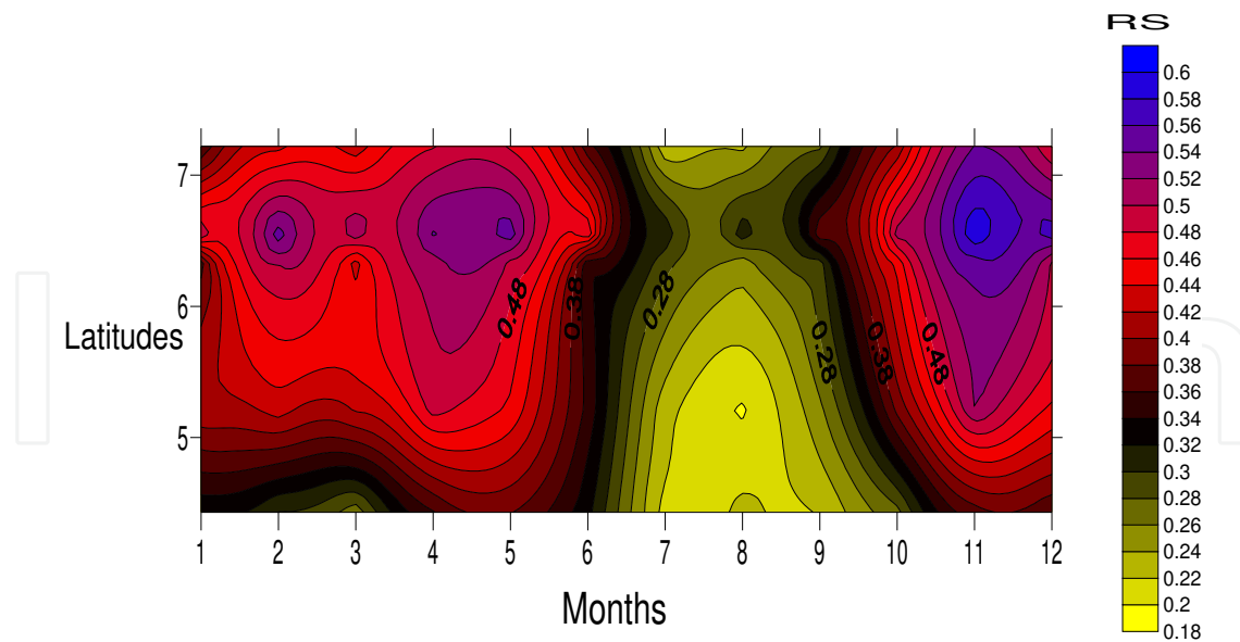
Fig. 3.4. Monthly variation of relative sunshine duration for selected stations (Ikeja, Ilorin, Ibadan, Port Harcourt and Benin).
