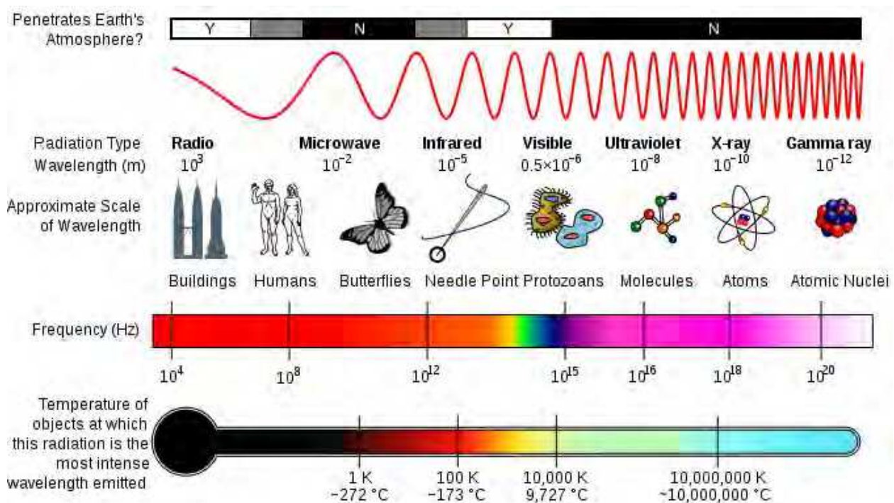
Fig. 1.2. Spectral ranges of electromagnetic radiation
