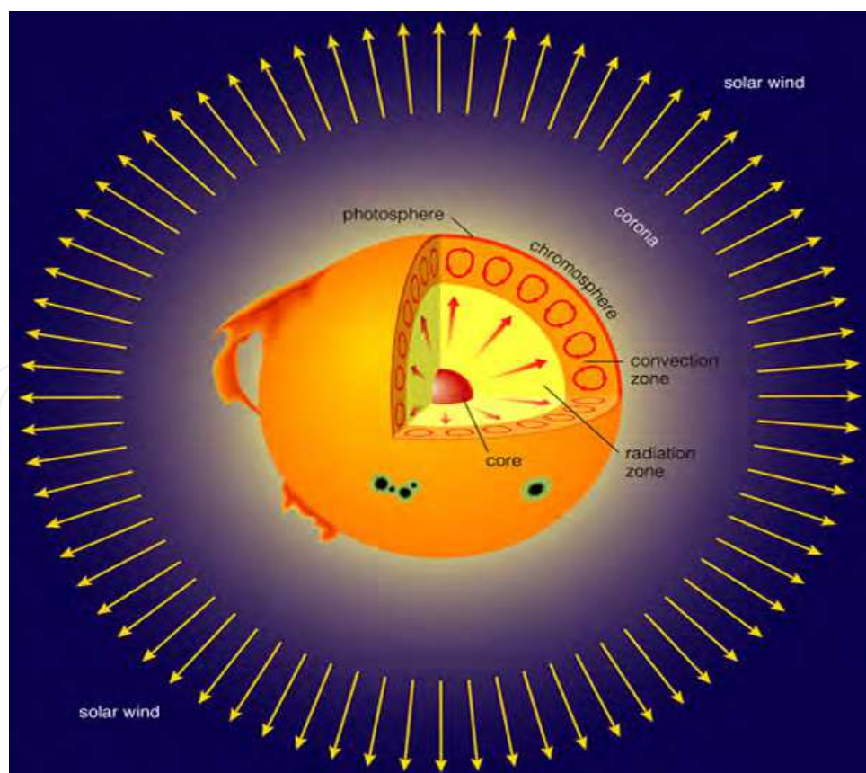
Fig. 1.1. The structure of the Sun
