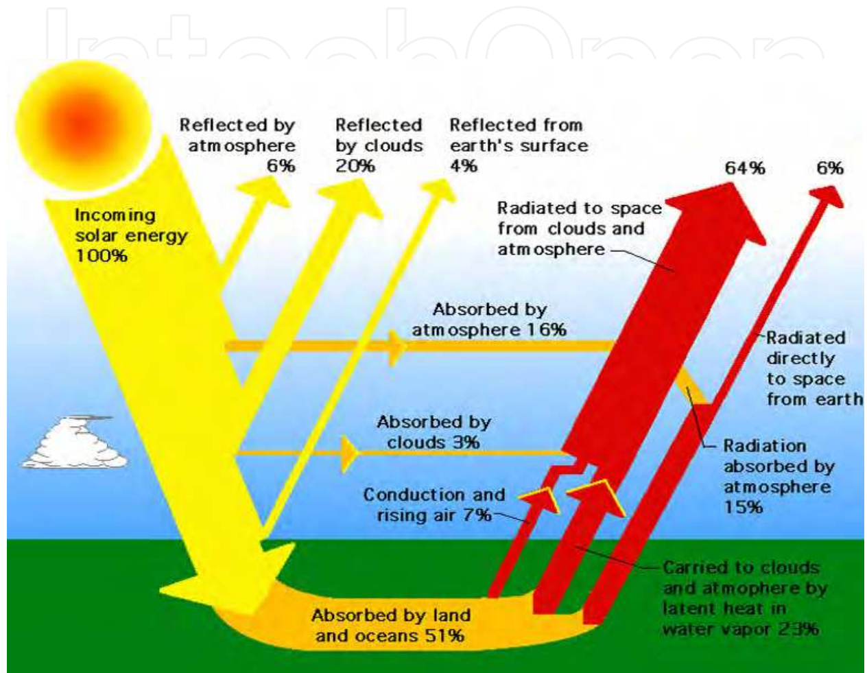
Fig. 1.3. Radiation balance of the atmosphere
