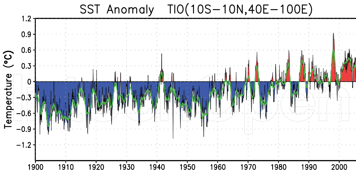
Fig. 1. Time series of the SST anomaly [ ^{\circ}\text{C} ] averaged in the tropical Indian Ocean ( 10^{\circ}\text{S} - 10^{\circ}\text{N} , 40^{\circ}\text{E} - 100^{\circ}\text{E} ). The SST data set is based on COBE-SST (Ishii et al., 2005). The red (blue) shaded area denotes positive (negative) anomalies. The base period is from 1971 to 2000.
