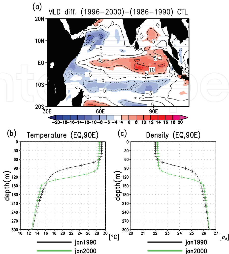
Fig. 3. (a) Mixed layer depth difference [m] between the 1996-2000 mean and the 1986-1990 mean. The shaded area denotes where the difference is positive. (b) Vertical profile of temperature [ ^{\circ}\text{C} ] in the equatorial Indian Ocean in CTL on January 1990 (black) and on January 2000 (green). (c) Same as (b) but for potential density [ \sigma_\theta ].
