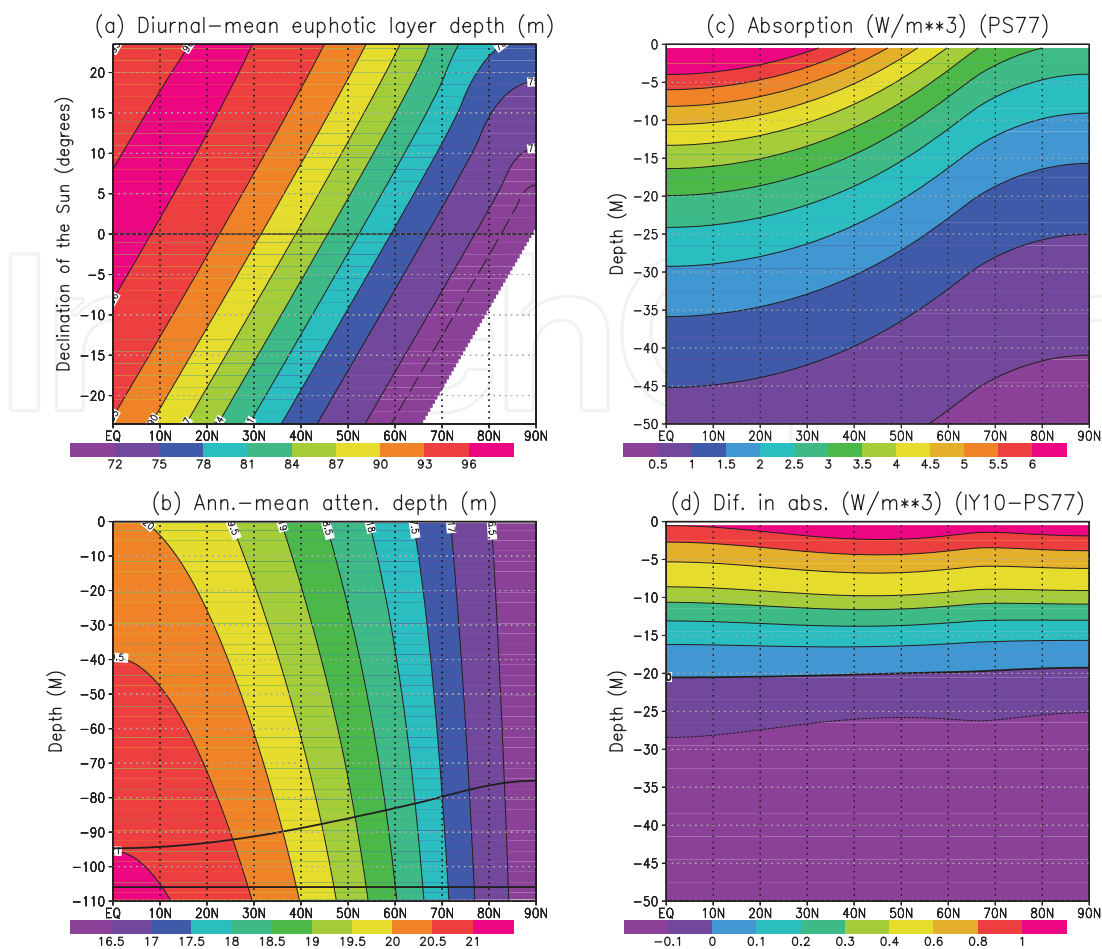
Fig. 6. (a) Diurnal-mean euphotic layer depth d_e [m] for IY10, for the sun declination \delta and the northern latitude \theta . (b) Meridional section of the effective attenuation depth \zeta [m] defined in each 1 m-layer for annually averaged diurnal-mean penetrating irradiance of IY10. (c) Absorption of annually averaged irradiance of PS77 [ \text{W m}^{-3} ]. (d) Difference in absorption between IY10 and PS77 [ \text{W m}^{-3} ] (IY10 - PS77). The thick lines in (b) indicate the annual mean euphotic layer depth for IY10 and PS77 (constantly 105.9 m).
