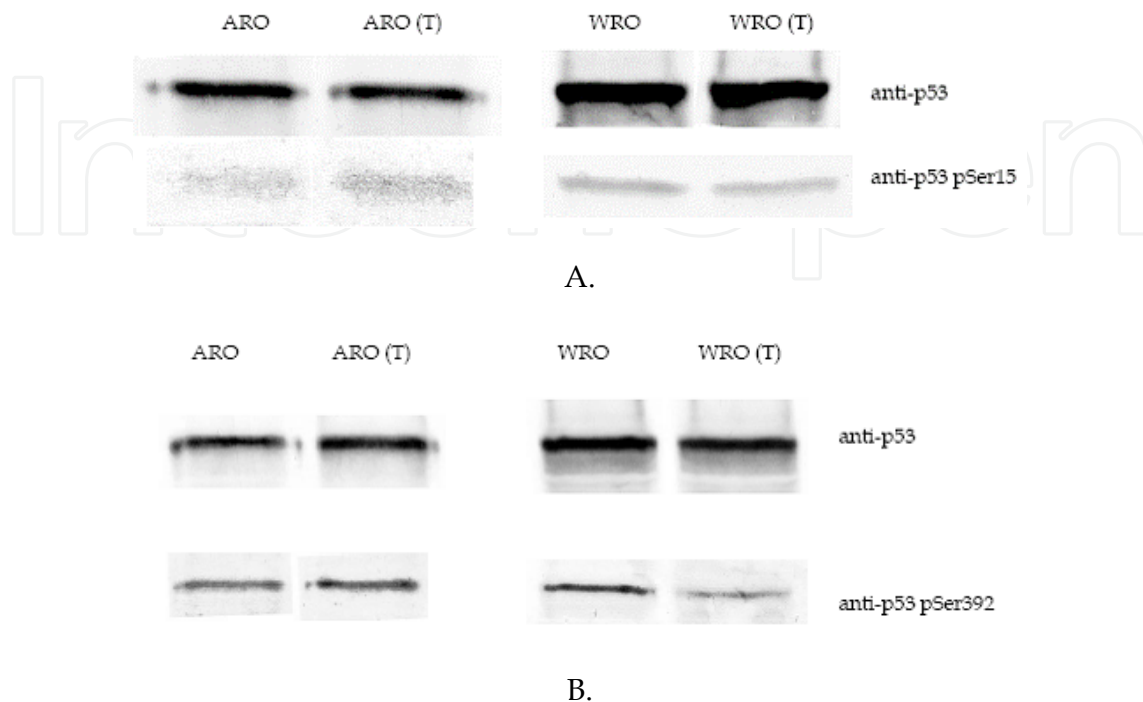
Fig. 3. Western blot analysis of the phosphorylation state of p53 at residues 15 and 392. Nuclear extracts from ARO and WRO thyroid cancer cells containing 300pg of p53 (based on ELISA) were loaded on the gel, and the derived blot probed with antibodies to phosphorylated p53 at S15 (panel A) or at S392 (Panel B) and for total p53 (anti-p53). Phosphorylation of p53 at S15 does not appear to change in response to H 2 O 2 treatment, while that modification at S392 appears to decrease after treatment (for WRO cells only).
