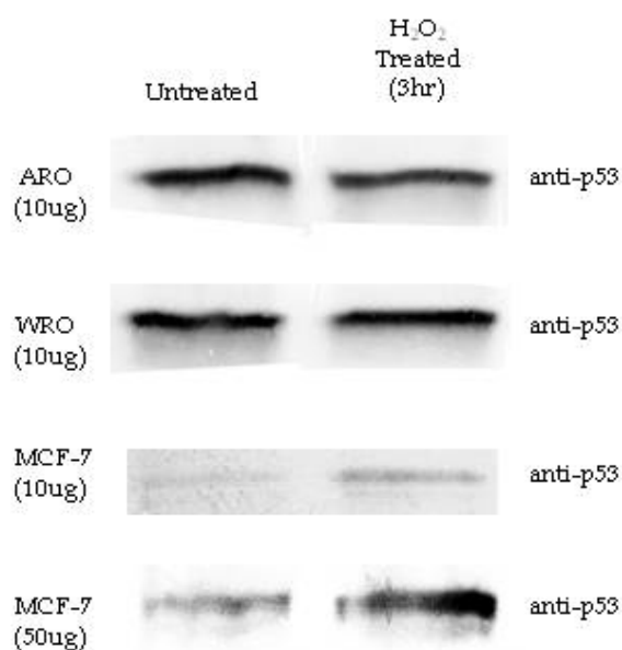
Fig. 2. Levels of p53 in nuclear extracts following H 2 O 2 treatment. Western blots were used to monitor the level of p53 in nuclear extracts of ARO, WRO and MCF-7 cells initially (untreated) and following a 3 hour treatment with H 2 O 2 . Total protein amount of 10 \mu g or 50 \mu g was loaded into each well. The level of p53 does not change in ARO and WRO mutant thyroid cancer cells upon treatment, while the amount of p53 increases in MCF-7 cells after H 2 O 2 treatment.
