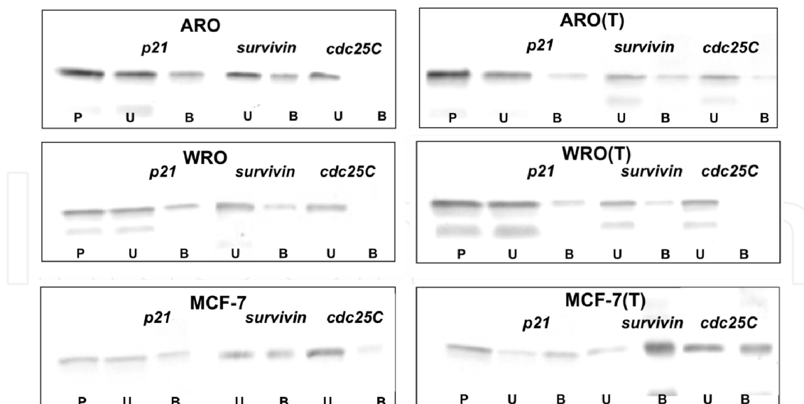
Fig. 4. DNA binding by p53 from nuclear extracts to various DNA sequences. DNA binding by 50pg of p53 to 20pmole biotinylated DNA sequences from the p21 , survivin , and cdc25C promoter regions were performed. The p53 in the DNA bound (B) or unbound (U) fractions and an equivalent aliquot of the protein prior to binding (P) were detected using western blots. Nuclear extracts were derived from ARO, WRO and MCF-7 cells, untreated and following H_2O_2 treatment (T). DNA binding occurs to the p21 and survivin gene promoters while no binding is detected to the cdc25C gene by the p53 from the ARO and WRO cells. Binding is detected to all of the sequences by the p53 from the MCF-7 cells, which increases upon treatment with H_2O_2 .
