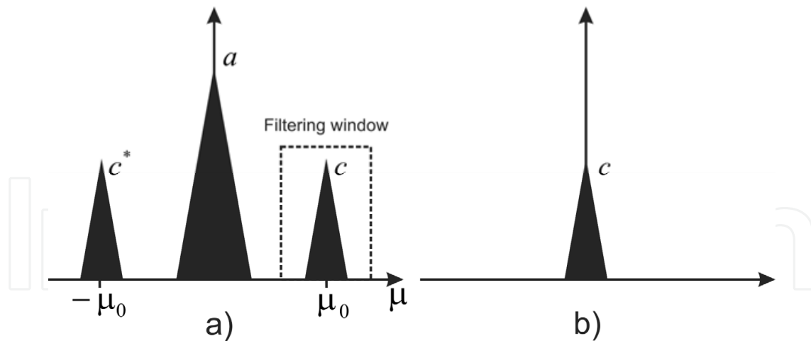
Fig. 4. a) Intensity distribution obtained with the FT of the interference pattern, b) spectrum translated to the origin.
