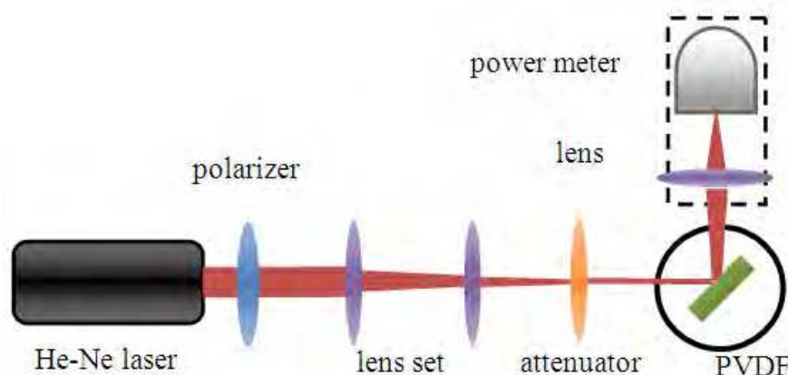
Fig. 16. Configuration of PVDF Brewster angle measurement.
