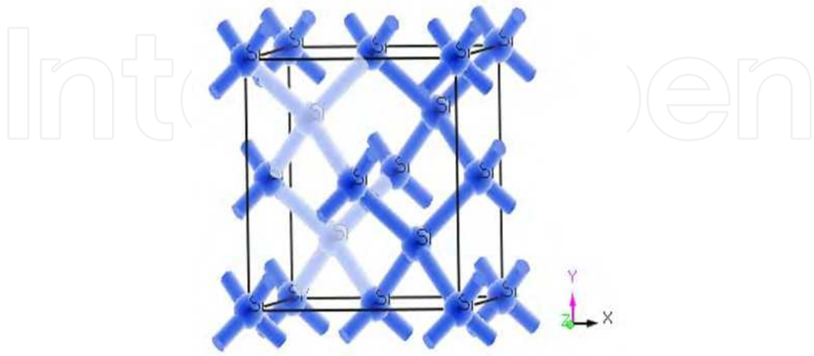
Fig. 6. Unit cell of the modified Si crystal with two vacancies (Space group: FD-3M (227); Lattice parameters: a: 5.43, b: 5.43, c: 5.43; \alpha: 90^\circ , \beta: 90^\circ , \gamma: 90^\circ ).
