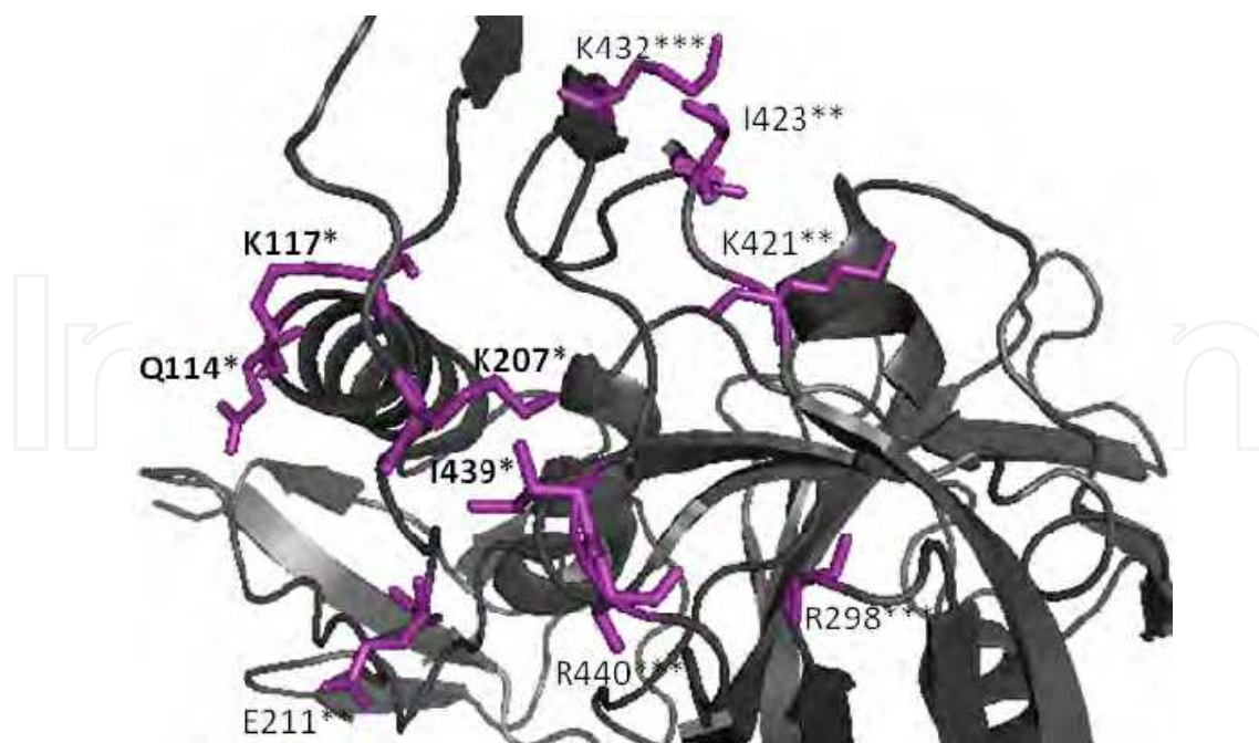
Fig. 9. A ribbon diagram of gp120 highlighting amino acid residues that interact with B40 aptamer. Residues in bold and single asterisk are highly conserved among all HIV-1 isolates and significantly reduced binding of the aptamer by more than 10-fold when experimentally mutated to alanine, respectively (Joubert et al. , 2010). Those residues with double or tripple asterix are moderately and significantly varaiable, respectively, in all HIV isolates and while they make contact with the aptamer they did not significantly affect binding of the aptamer when experimentally mutated to alanine, respectively.
