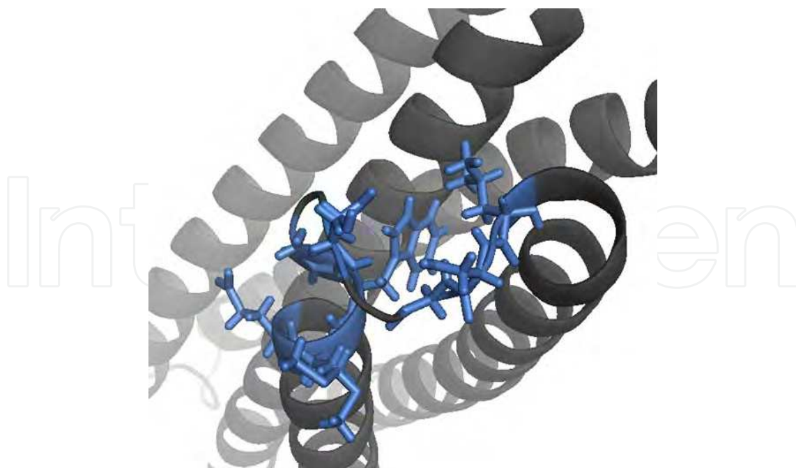
Fig. 6. Ribbon representation of HIV-1 heptad repeat fusogenic domain showing point mutations (colour coded blue) that cause resistance to fusion inhibitors.
