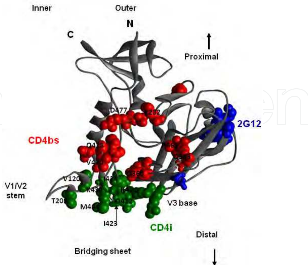
Fig. 8. Ribbon diagram illustrating epitopes of the gp120 core, highlighting some amino acid residues that interact with broadly neutralizing antibodies. The CD4bs (red) and the CD4i co-receptor-binding surface (green) as well as residues implicated in 2G12 binding (blue) are depicted.
