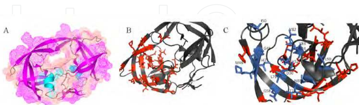
Fig. 4. Bound crystal structure of HIV-1 protease showing the residues where major PI-resistance mutations occur. (A) Mesh illustration of HIV-1 protease in bound state with saquinavir. (B) Illustration of amino acid residues (colour coded red) where PI-resistance point mutations occurs. (C) Zoomed-in illustration showing in detail residues (colour coded blue) where major PI-resistance mutations occur.
