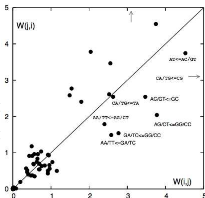
Fig. 3. The dinucleotide replacement probabilities W(i,j) presented in the same way as the A(i,j) counts in Fig. 2. Note that the italicized dinucleotide pairs exhibit the opposite directionalities in comparison with the A(i,j) values. The CA/TG \rightleftharpoons CG replacement probabilities are located in the direction indicated by the two arrows at x=21 (horizontal arrow) and y=21 (vertical arrow). The units are arbitrary.
