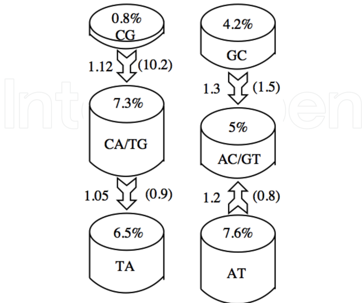
Fig. 5. The asymmetries of the GC, AC/GT, AT, CG, CA/TG and TA replacements. See also the caption of Fig. 4.
