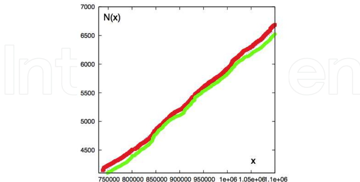
Fig. 9. Red squares and green circles represent the counts of nucleotide replacements taking place in human and chimpanzee species, respectively, as a function of the first chromosome coordinate x .
