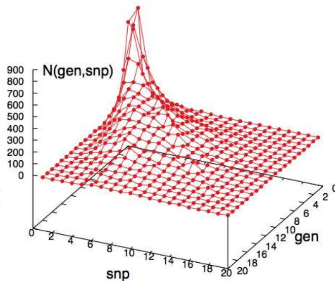
Fig. 7. A three dimensional plot of the genomic and snp type nucleotide replacement densities. The coordinates of the points in two horizontal directions have the following meaning: number of genomic replacements per 1000 nucleotides for the “gen” direction and number of snp nucleotide replacements per 3800 nucleotides for the “snp” direction. The heights of the points represent the number of segments having the densities specified by the two horizontal coordinates.
