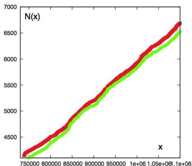
Fig. 8. Red squares, green circles and blue triangles (hidden behind the red squares) represent the counts of nucleotide replacements and repeat elongation/shortening of mononucleotide and dinucleotide repeats, respectively, as a function of the first chromosome coordinate x .
