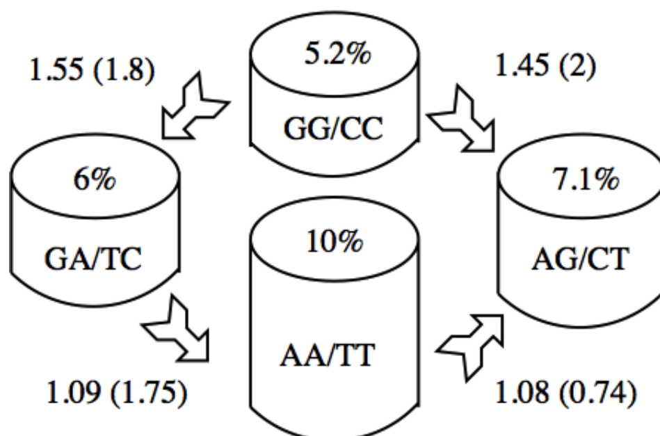
Fig. 4. The asymmetries of the GG/CC, GA/TC, AG/CT replacements. The height of the barrels is proportional to their composition (given in percents at the top). For each replacement the arrow shows the predominant directionality. The numbers beside the arrows give the asymmetry factor - the A_{ij}^{(d)}/A_{ji}^{(d)} ratio. The numbers in parentheses give the corresponding W_{ij}/W_{ji} ratios.
