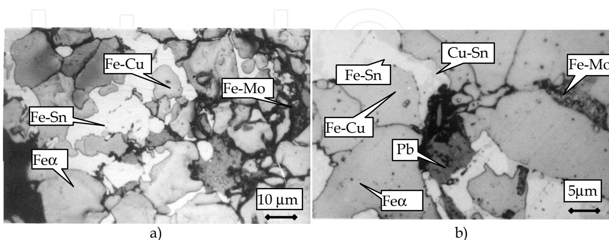
Fig. 10. Microstructure of the MAS1 (a) sintered at 800°C/20min and MAS2 (b) sintered at 850°C/50min.
