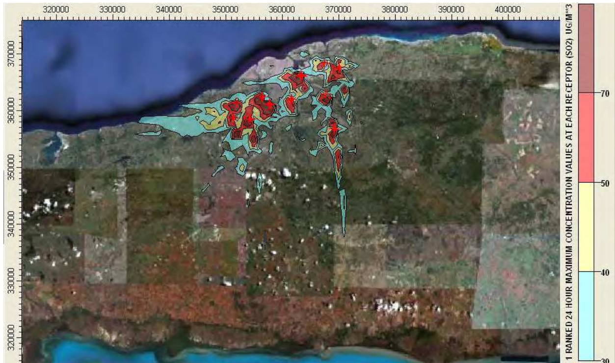
Fig. 6. Isolines of the maximum hourly concentration of SO 2 . (Source: Base Map Google Earth)
