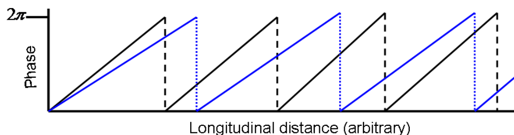
Fig. 20. Phase maps for two wavelengths.
