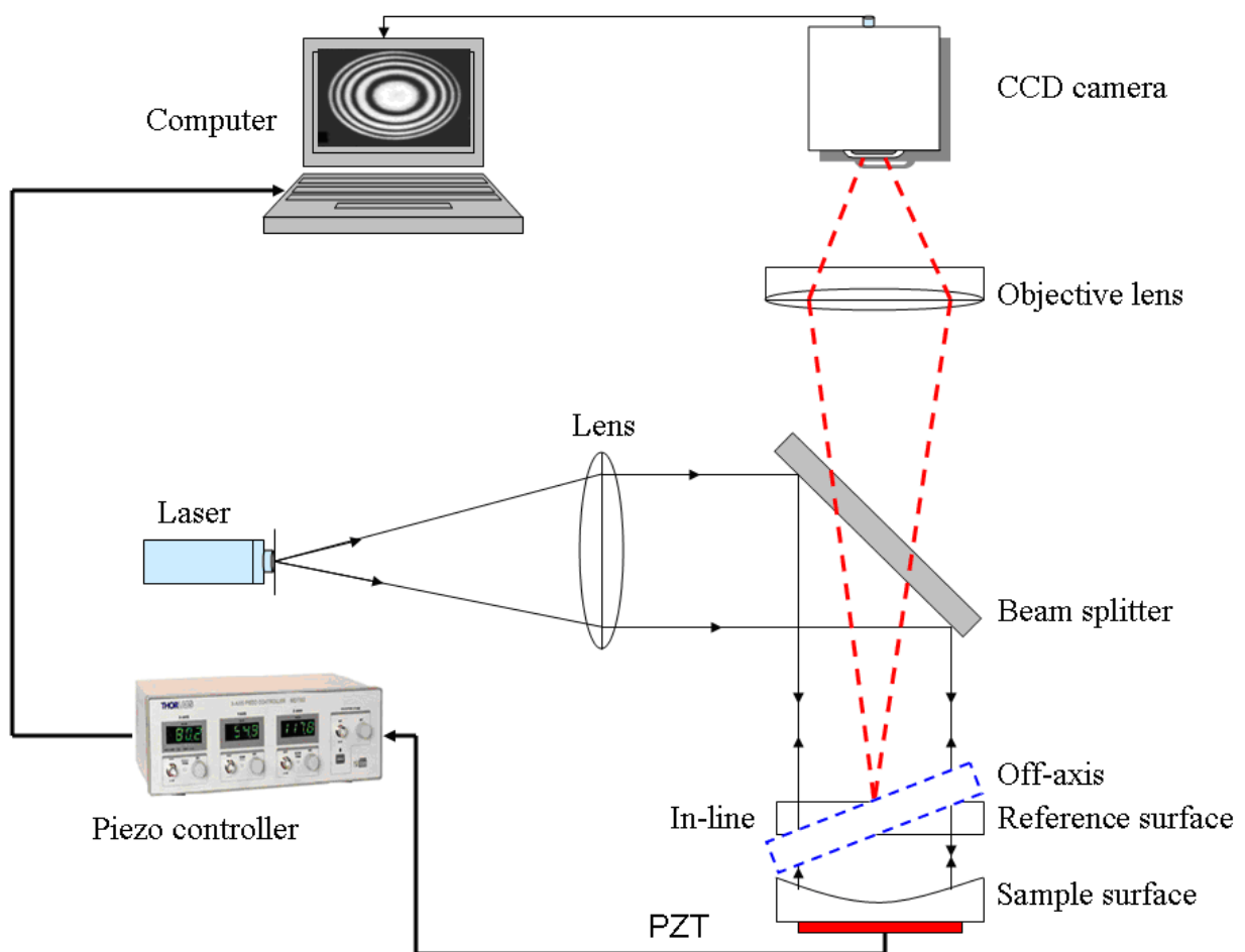
Fig. 6. Schematic diagram of the optical setup.
