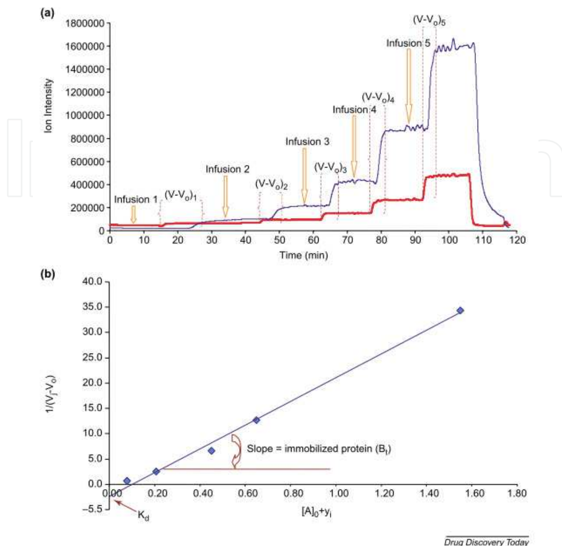
Fig. 4. Depiction of a typical 'modified staircase' experiment to evaluate K_d for a protein target (immobilized in the column) and a small molecule ligand. (a) The ligand (blue) is infused at increasing concentrations starting from an initial (i) to a final (j) concentration along with a void marker (red). (b) The reciprocal of the breakthrough volumes, 1/(V_j-V_0) , are plotted against the summed ligand concentrations, [A]_0+y_j , to produce a linear correlation from which the K_d value can be determined from the y intercept. The total amount of immobilized protein ( B_i ) in the column is then obtained from the slope .
