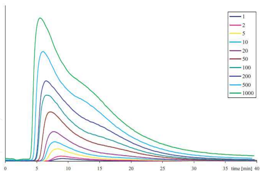
Fig. 7. The effect of increasing concentrations of mecamlamine, from 1 to 1,000 mM, on the chromatographic profiles of mecamlamine. For experimental details, see reference (Jozwiak et al., 2002).
