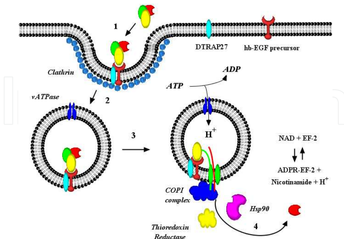
Fig. 2. Schematic Overview of DT Intoxication. (1) DT binds to its cell surface receptor (2) Internalization of clathrin coated pits into early endosomal vesicles (3) Acidification of the endosomal lumen induces DT T domain insertion and pore formation (4) Translocation and cytosolic release of the DT C domain is facilitated by COPI complex, Thioredoxin Reductase and Hsp90. Refolded DT C domain catalyzes the ADP-ribosylation of EF-2. Diphtheria toxin: yellow = receptor binding (R) domain; green = transmembrane (T) domain; red = catalytic (C) domain. Reproduced from Murphy (2011).
