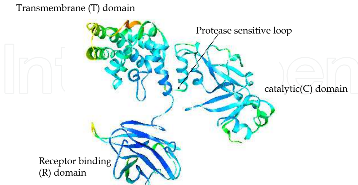
Fig. 1. X-Ray Crystallographic Structure of Diphtheria Toxin. PDB 1 MDT. Modified from Choe et al., 1992.
