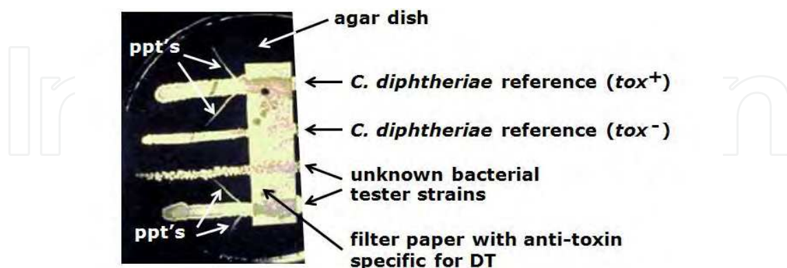
Fig. 3. The Elek immunodiffusion test. Shown is an agar plate with an antitoxin soaked filter that is inoculated with known toxigenic ( tox + ) and non-toxigenic ( tox - ) isolates of C. diphtheriae and unknown bacterial tester strains. The thin white lines (arrows) represent anti-toxin/DT precipitates ("ppt's") indicating bacterial DT production. Permission to show Rahul Gladwin's blog data ( http://www.rahulgadwin.com/noteblog/bacteriology/what-is-an-eleks-test.php ) is acknowledged.
