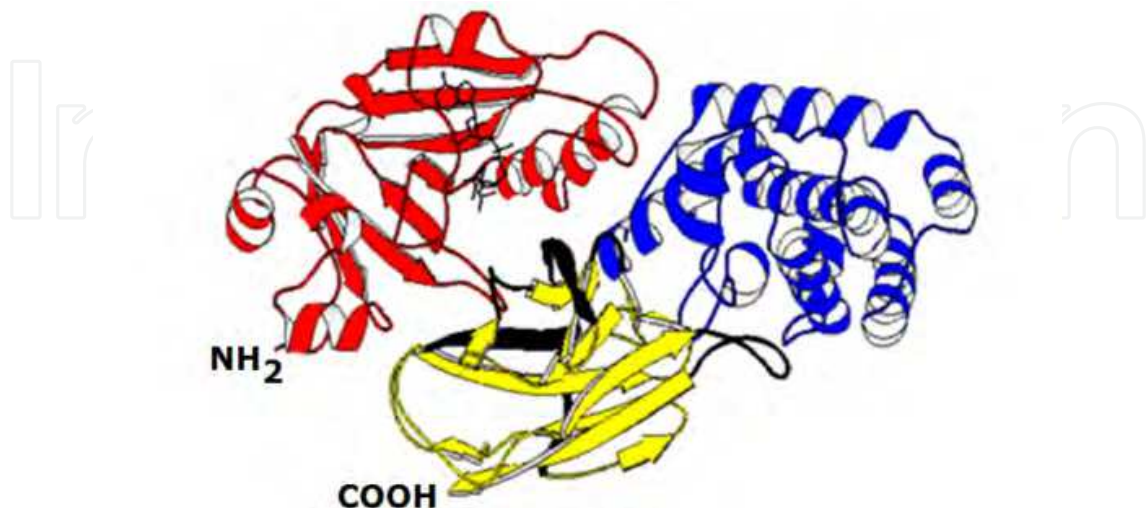
Fig. 5. MolScript-based ribbon diagram highlighting the modular domain organization of the DT monomer. The amino and carboxyl termini of full length DT are indicated ( \text{NH}_2 and \text{COOH} , respectively). The domain in red represents the N-terminal ADP-ribosyltransferase catalytic centre which accounts for cytotoxic ADP-ribosylation and inactivation of the DT target protein EF2; the yellow motif illustrates the C-terminal binding domain important for cell surface attachment and receptor-mediated endocytosis of DT; the protein domain in blue is the transmembrane motif responsible for endosome insertion and subsequent subcellular release of the cytotoxic ADP-ribosylase domain. Permission by Professor Kenneth Todar, University of Wisconsin, USA, to reproduce a modified version of the illustration (Todar, 2004) is gratefully acknowledged.
