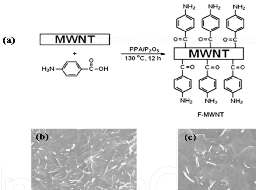
Fig. 5. (a) Schematic of the Side-wall functionalization of MWNTs (F-MWNTs) by Friedel-Crafts acylation, (b) SEM images of the fractured surfaces of a P-MWNT (5 wt%)/nylon-6 and (c) F-MWNT (5 wt%)/nylon-6 (Saeed et al., (2009)
