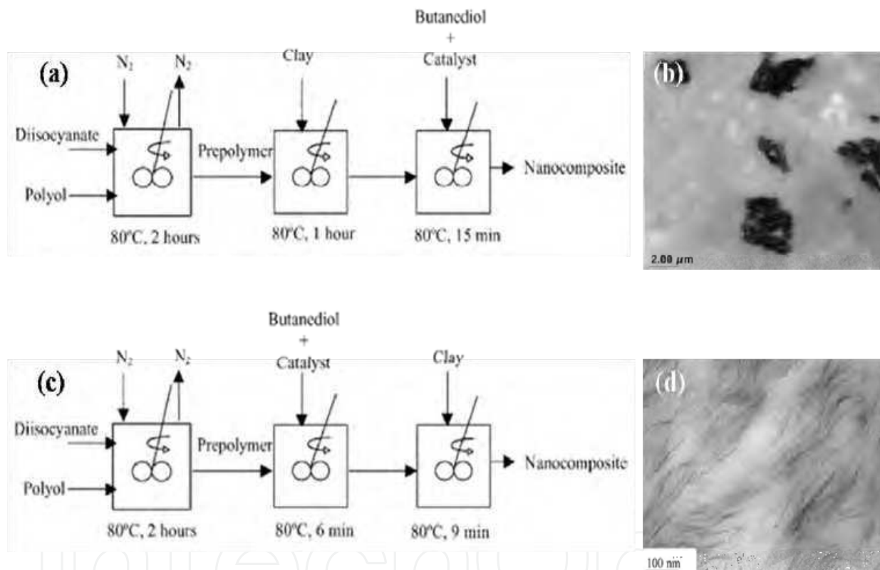
Fig. 3 Schematics of clay/polyurethane nanocomposite preparation and their respective TEM images; (a) method I and (b) TEM image of 4 wt% clay/polyurethane nanocomposite prepared by method I, (c) method II and (d) TEM image of 5 wt% clay/polyurethane nanocomposites prepared by method II.
