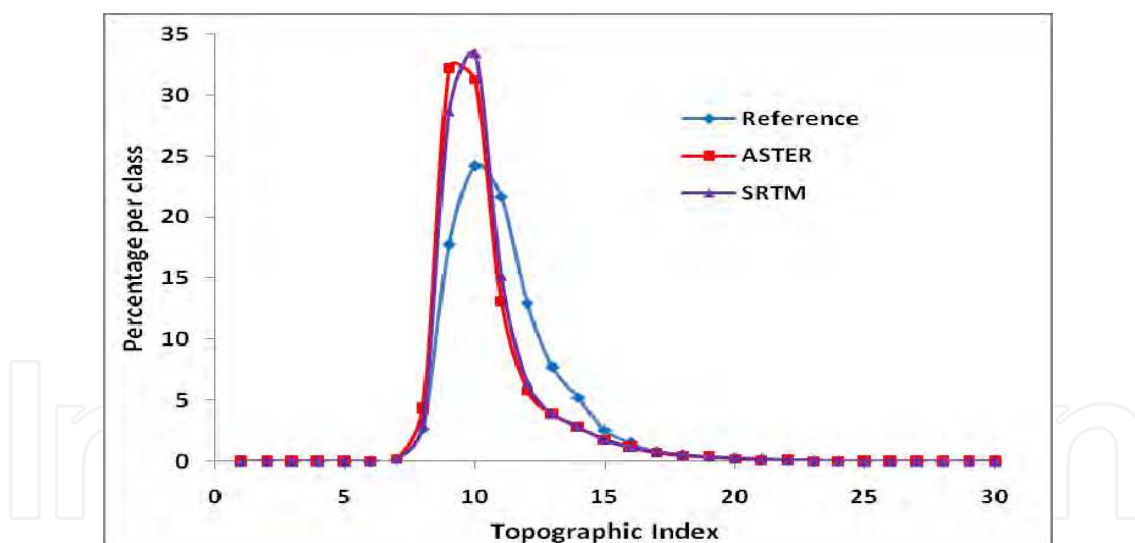
Fig. 8. Comparison of Topographic Index classes for the DEM's
