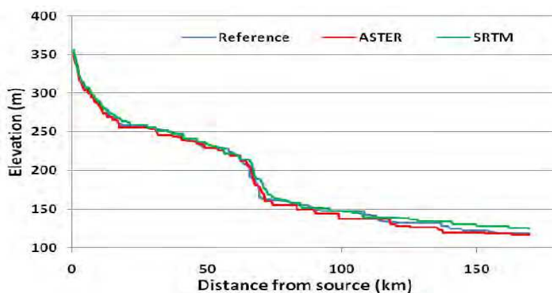
Fig. 5. Longitudinal profiles extracted from the three DEMs
