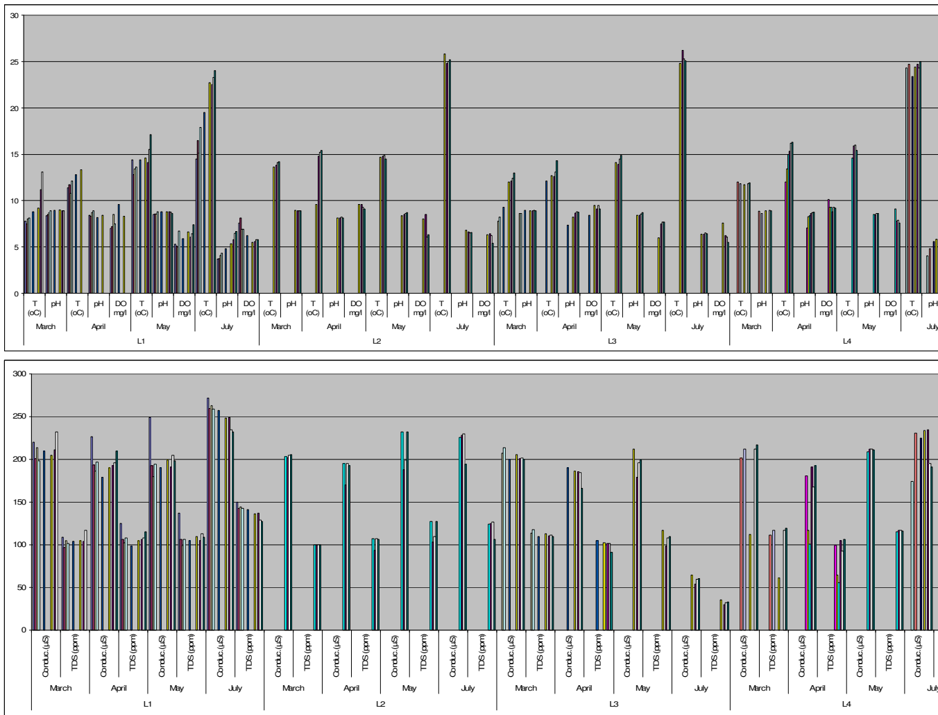
Fig. 24. Basic physical parameters detected at Prespa Lake sampling sites. The above findings are additionally complemented by dissolved oxygen results. Deep water layers had showed relatively high DO values in the summer months, their values even exceeded those of the upper water layers. Maximal DO values were recorded at around 3-4 m depth layers where the phytoplankton was in its peak. These results are sharply opposite to frequent statements of oxygen depletion in the deep water layers of Prespa Lake. The lowest DO values during our investigations were 5-5.3 mg·L -1 at the deepest part of the L1 sampling site in May 2010.
