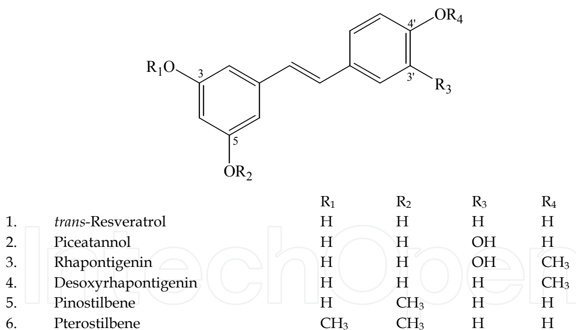
Fig. 1. Structure of trans -resveratrol and its natural analogues
