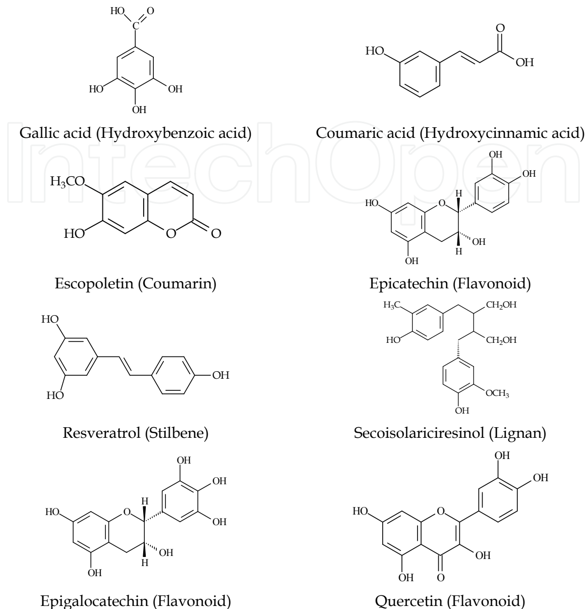
Fig. 1. Chemical structures of some phenolic compounds.
