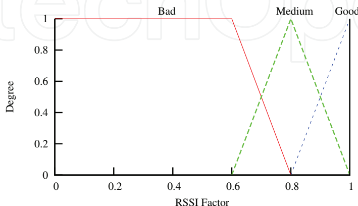
Fig. 6. Signal strength membership function.
