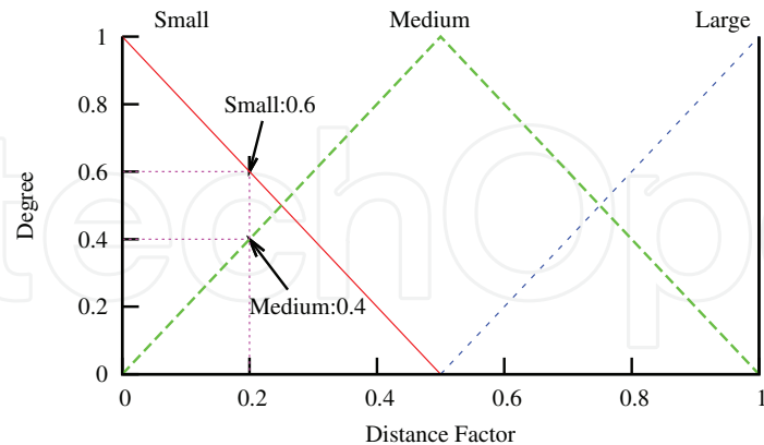
Fig. 4. Distance membership function.
