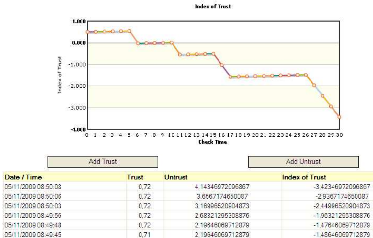
Fig. 7. Trust variation with trust restrictions.
