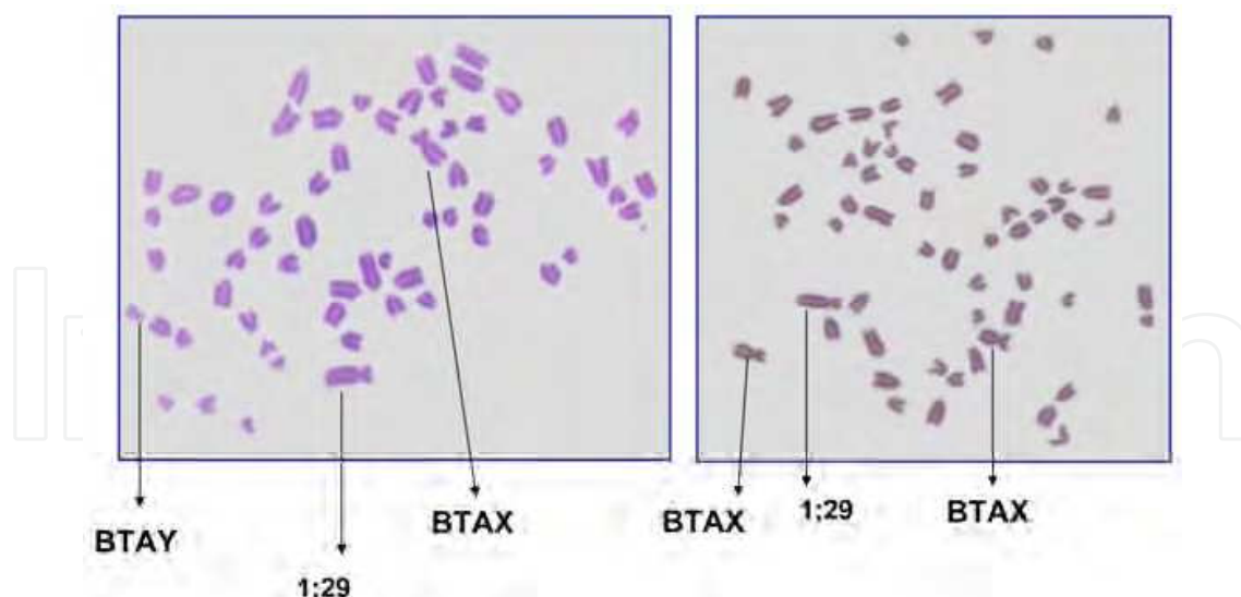
Fig. 2. Lymphocyte metaphases of male and female cattle carriers of rob(1;29) (courtesy: Iriarte, W., 2008).
