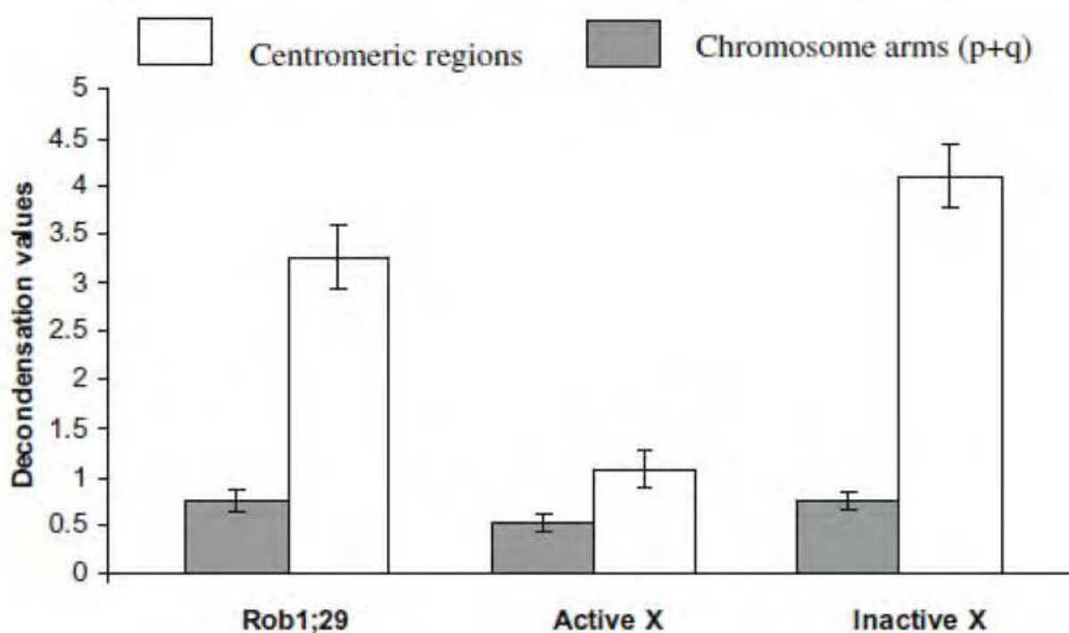
Fig. 7. Effects of 5-Aza-C on biallelic chromosome of rob(1;29) carrier cow. Histograms depict average decondensation values and standard errors in centromeric regions and chromosome arms (p + q) for rob(1;29); active and inactive X chromosomes.
