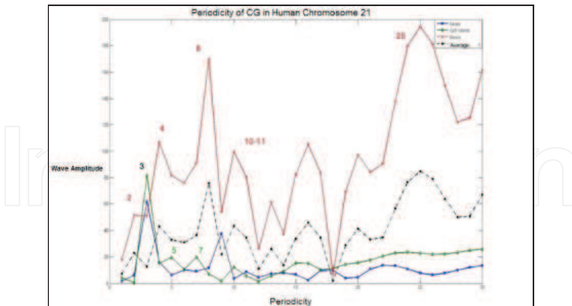
Fig. 2. Fourier analysis (Periodicity Vs Average Wave Amplitude) of global periodicities of CG dinucleotides in 19 Genes (blue line), non-coding near them (red line) and all CpG Islands (green line) in chromosome 21. The average of the 3 region levels is shown as a dotted line.
