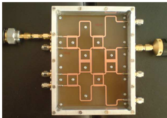
Fig. 10. Fabricated 4x4 ITS Butler Matrix Microwave BFN.
