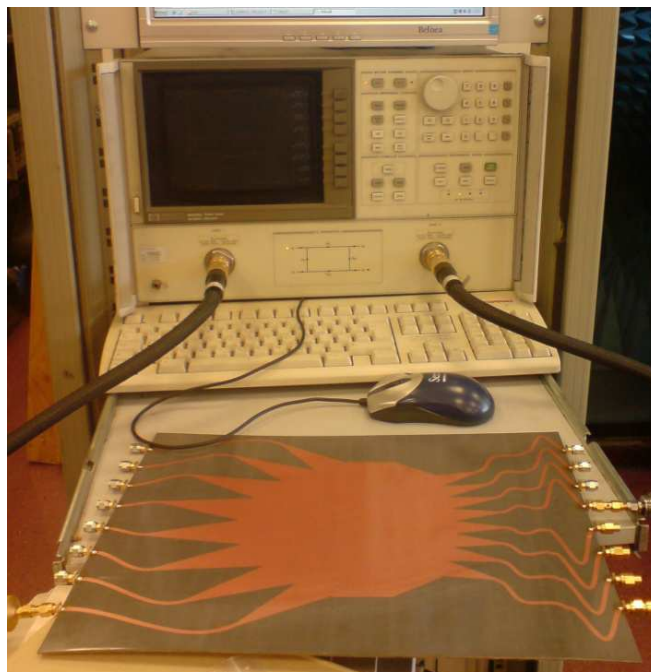
Fig. 6. Fabricated 8 \times 8 ITS Rotman Lens Microwave BFN.
