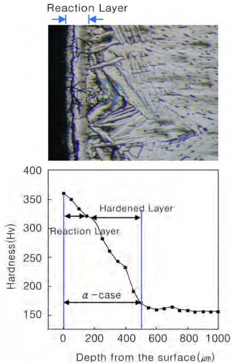
Fig. 3. Microstructure of the interface between Ti and \text{Al}_2\text{O}_3 mold, and hardness profile.
