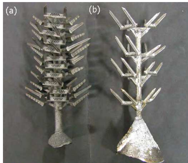
Fig. 12. Comparison of externals of titanium castings (a) CaO stabilized ZrO_2 mold and (b) the \alpha -case controlled stable mold.
