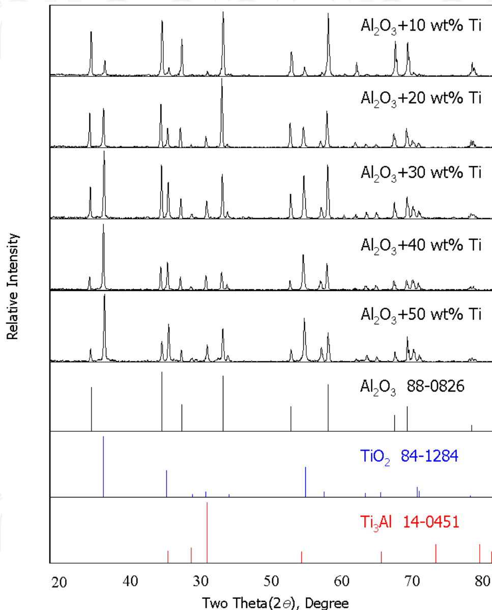
Fig. 11. Illustration of the diffraction patterns and replots for identifying phases from 10 wt% to 50 wt% titanium and \text{Al}_2\text{O}_3 after curing at 1,223 K for 2 hrs.
