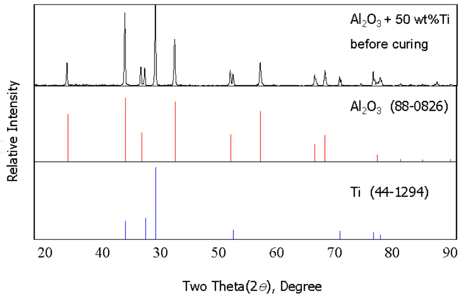
Fig. 9. Illustration of the diffraction patterns and replots for identifying phases in 50 wt% titanium and \text{Al}_2\text{O}_3 mixed with colloidal silica before curing.
