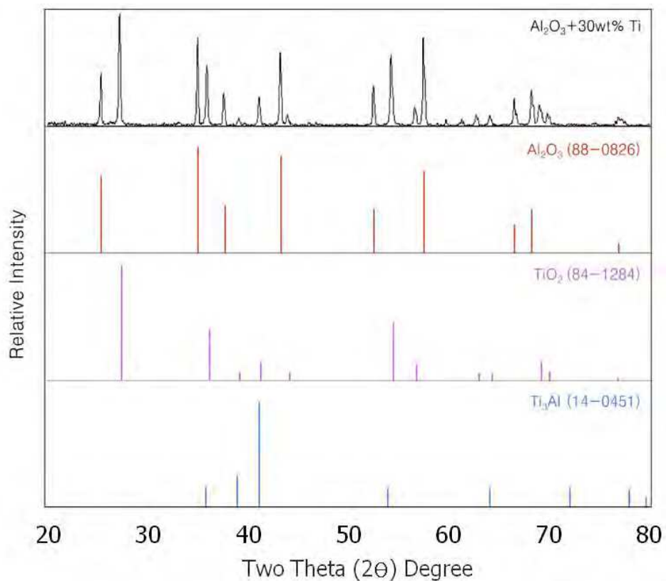
Fig. 10. X-ray diffraction pattern of synthesized \alpha -case controlled stable mold materials.
