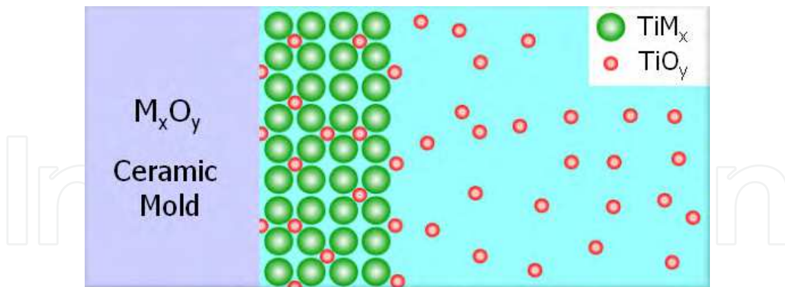
Fig. 8. Schematic diagram of the interstitial and substitutional \alpha -case formation mechanism of titanium castings.
