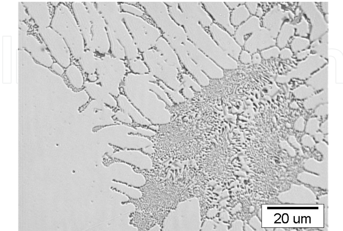
Fig. 5. Dendrites of primary \alpha_{Al} phase in the component.
