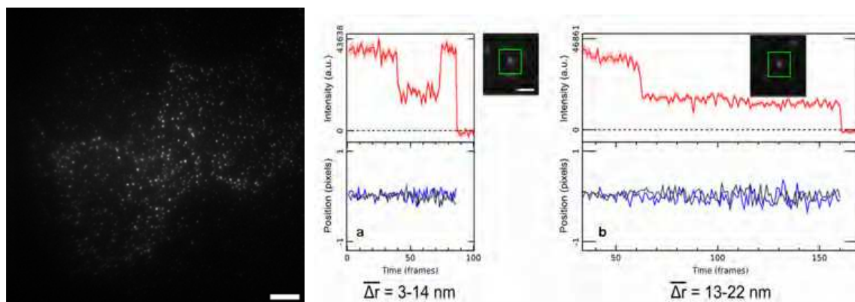
Fig. 7. Left: Single molecule TIRF image of EGFR in the plasma membrane of HeLa cells. EGFR are labelled with their ligand EGF, conjugated with the fluorophore Atto 647N (bar 8 \mu\text{m} ). Right: Traces of single molecule fluorescence intensity (red) vs time for two example spots in fixed HeLa cells labelled with EGF-Atto 647N. a) shows a relatively short intramolecular distance, b) a longer distance. Fluorophore x and y positions are plotted in black and blue, respectively.
