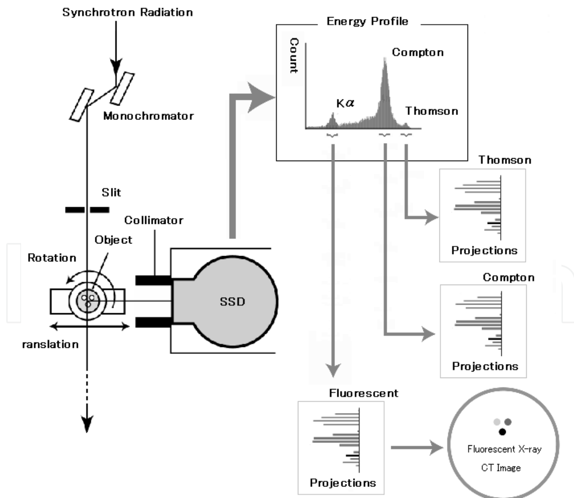
Fig. 9. Schematic of fluorescent x-ray CT system
