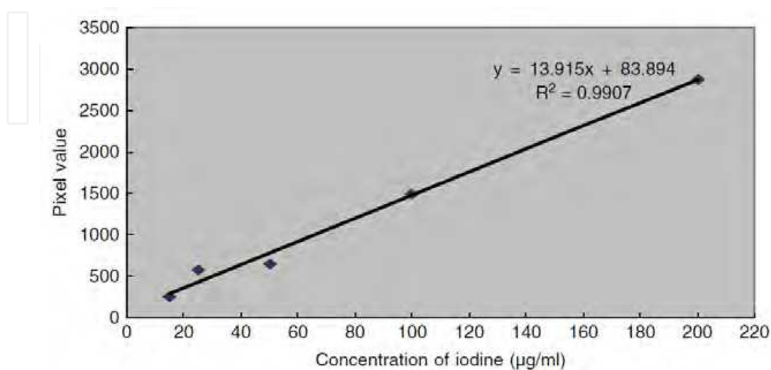
Fig. 20. Relationship between actual iodine concentration and FXCT pixel value.
