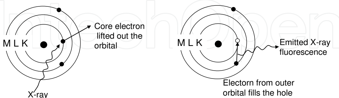
Fig. 1. Emission of fluorescent x ray
