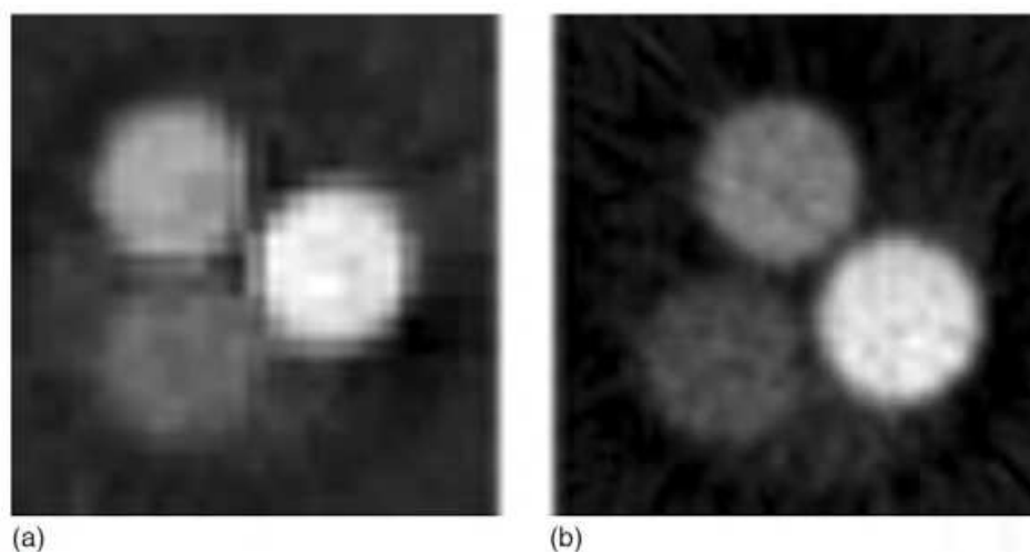
Fig. 19. FXCT image of a 10-mm-diameter acrylic cylindrical phantom which has three channels (3 mm \phi ) filled with three different concentrations of iodine solution: (a) coarse collimator, (b) fine collimator (Huo, et al., 2009).
