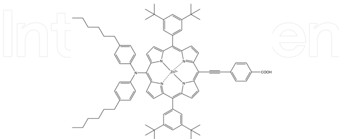
Fig. 5. Molecular structure of YD-2.
