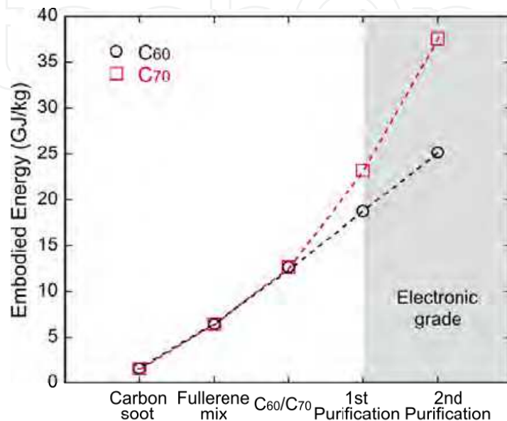
Fig. 7. Embodied energy for C_{60} and C_{70} products as a function of product stage (Anctil et al. 2011).
