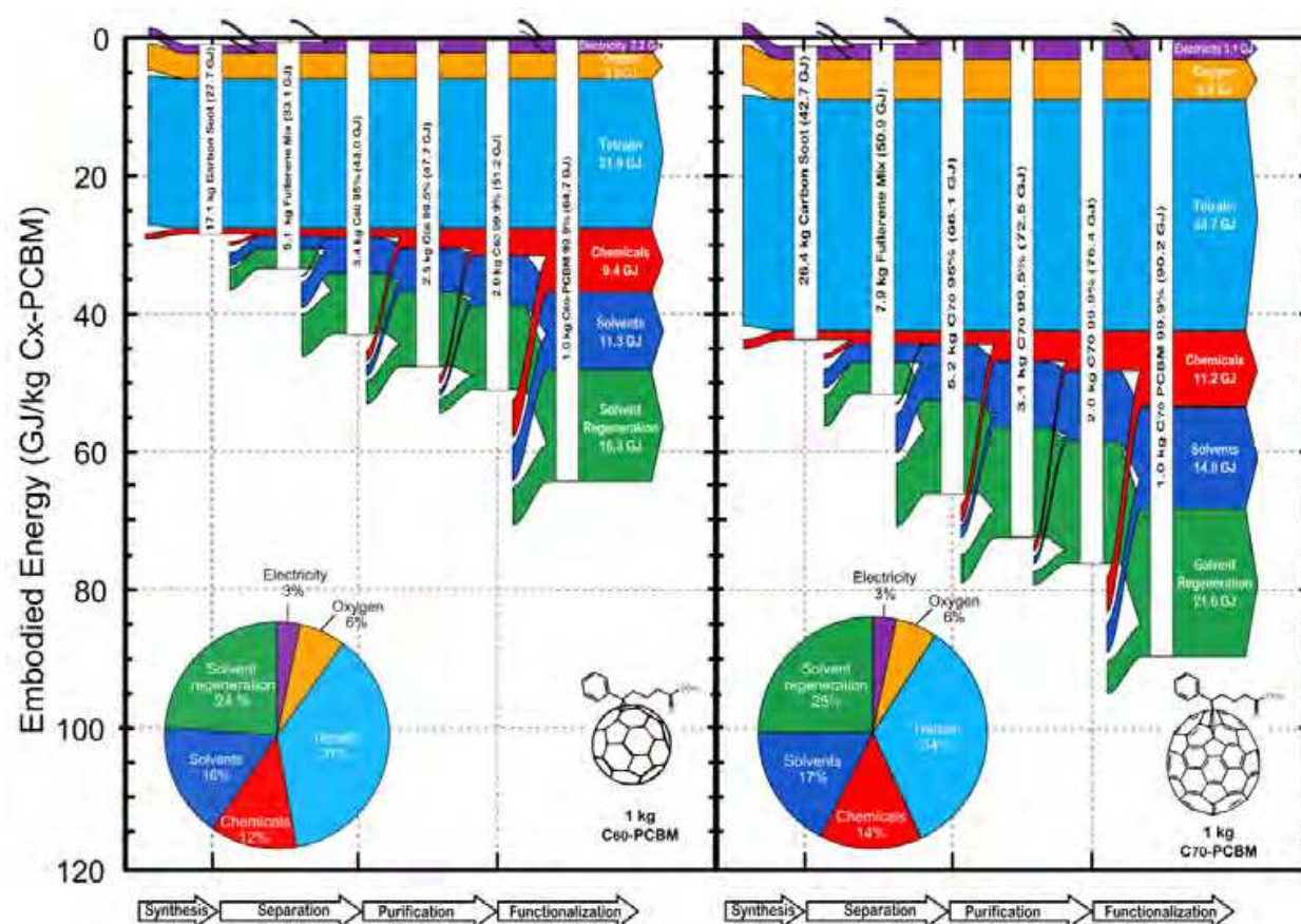
Fig. 8. Energy flow diagram for production using the pyro-tetralin synthesis method of (a) 1 kg of C 60 PCBM, compared to (b) 1kg of C 70 PCBM (Anctil et al. 2011).
