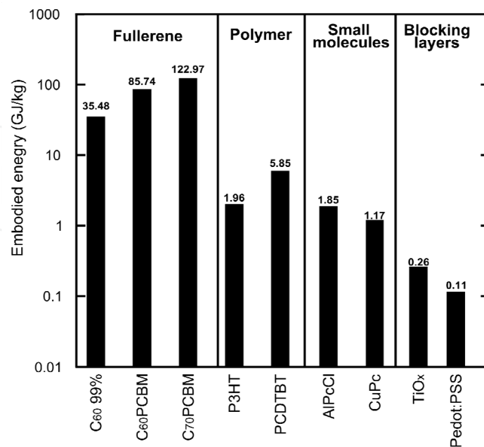
Fig. 10. Cumulative energy demand (CED) for various materials commonly used in organic photovoltaics.
