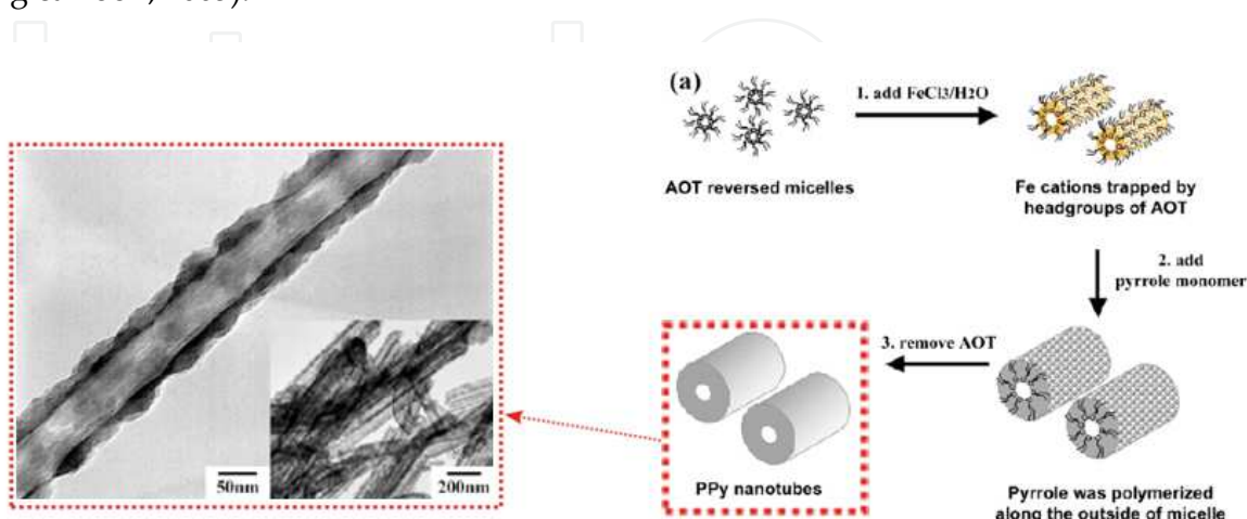
Fig. 3. TEM image and schematic route for the preparation of polypyrrole nanotubes in W/O microemulsion (Jang & Yoon, 2003)
