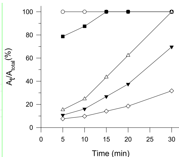
Fig. 5. Dispersation rate of mixture of Cremophor/Transcutol( S_{mix} ) (Cremophor EL®/Transcutol® as 0.5:1, 1:1, 2:1, 3:1, 4:1 and Captex 355 ( S_{mix} :Captex355=15:4) into aqueous media assuming the pH condition of gastric fluid.
