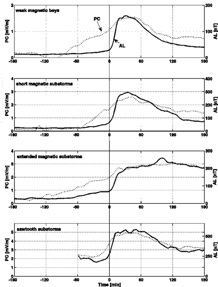
Fig. 6. Relationship between average PC and AL indices for weak magnetic bays (first panel), isolated short and extended substorms (second and third panels), and for sawtooth substorms (fourth panel) (Troshichev and Janzhura, 2009).
