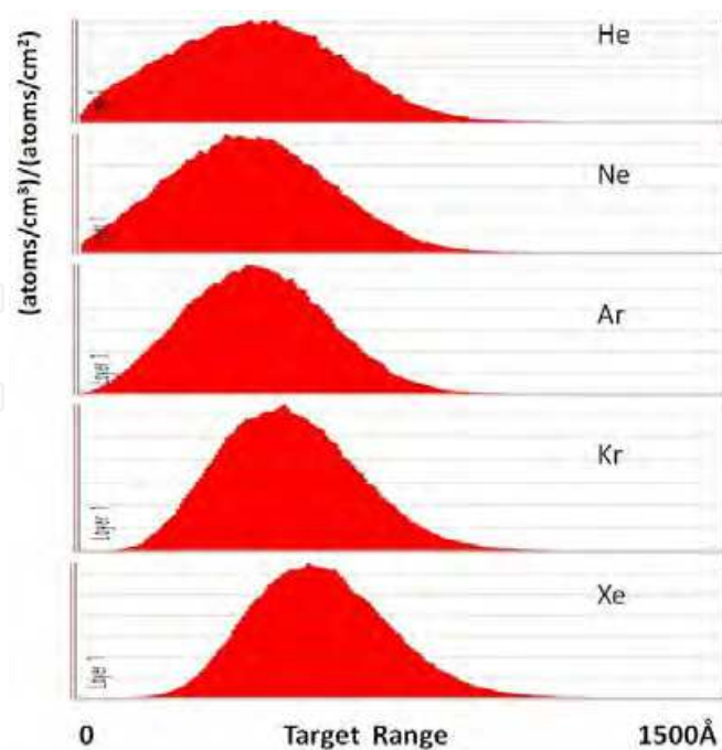
Fig. 1. Depth profiles of noble gases implanted into aluminum at 1\text{kV/nucleon} energy. Calculated by SRIM-2008 (Ziegler et al., 2008).
